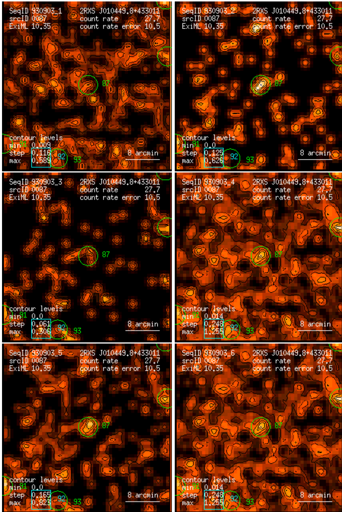
Figure 87: RASS 930903: detection 0087: band rate images, Gaussian filter: (1) PSPC channels 11 – 41, (2) 52 – 90, (3) 91 – 201, (4) 11 – 235, (5) 52 – 201, (6) 11 – 201. Broad band rates in counts/ks. Band rate contour levels in counts/ks/arcmin 2 .
