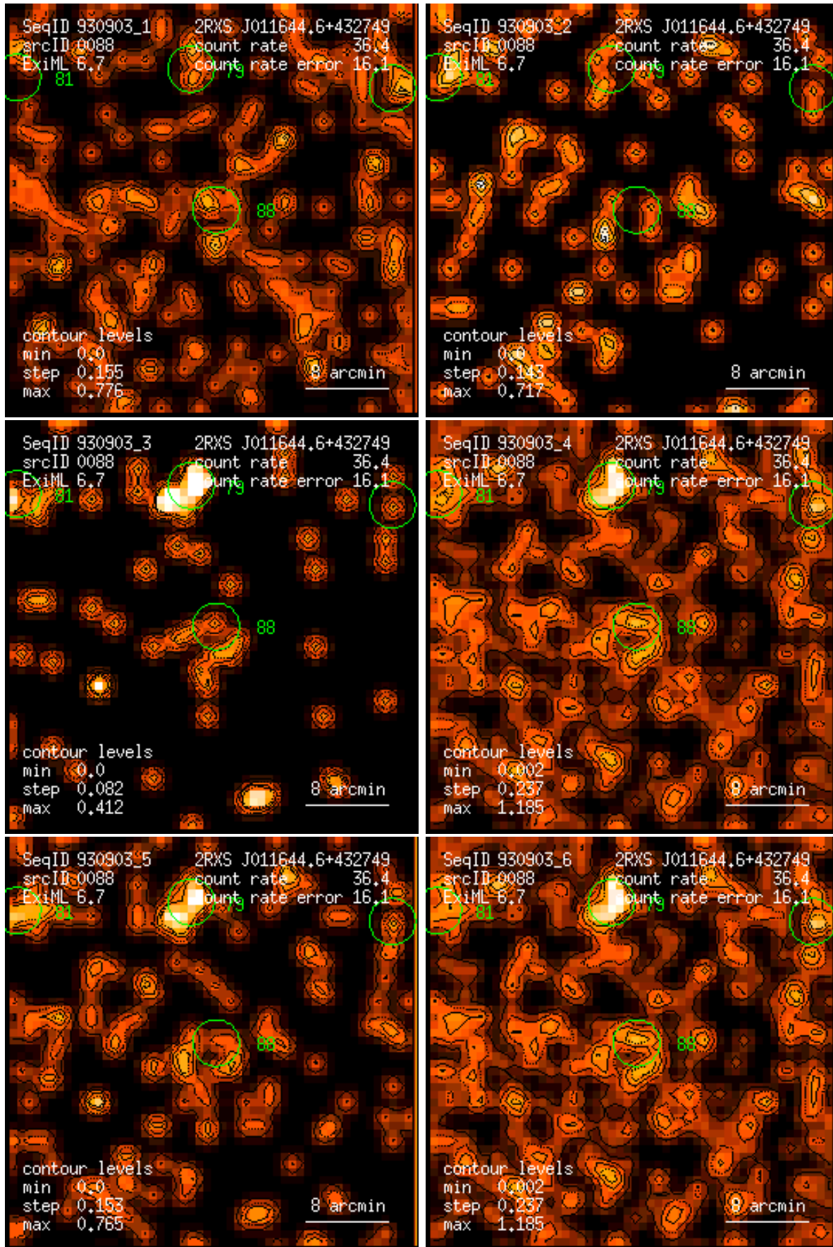
Figure 88: RASS 930903: detection 0088: band rate images, Gaussian filter: (1) PSPC channels 11 – 41, (2) 52 – 90, (3) 91 – 201, (4) 11 – 235, (5) 52 – 201, (6) 11 – 201. Broad band rates in counts/ks. Band rate contour levels in counts/ks/arcmin 2 .
