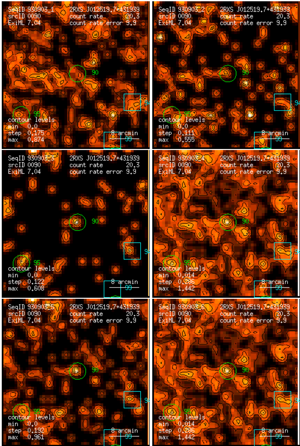
Figure 90: RASS 930903: detection 0090: band rate images, Gaussian filter: (1) PSPC channels 11 – 41, (2) 52 – 90, (3) 91 – 201, (4) 11 – 235, (5) 52 – 201, (6) 11 – 201. Broad band rates in counts/ks. Band rate contour levels in counts/ks/arcmin 2 .
