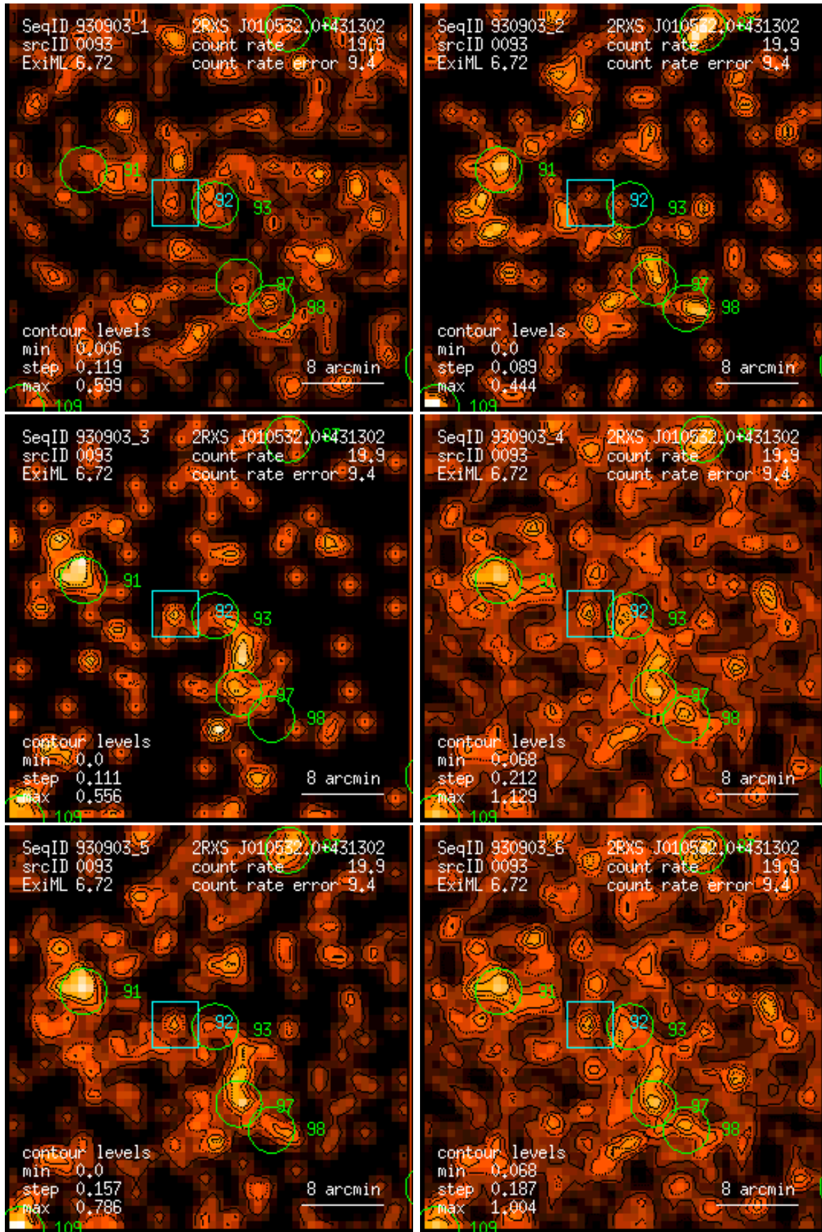
Figure 93: RASS 930903: detection 0093: band rate images, Gaussian filter: (1) PSPC channels 11 – 41, (2) 52 – 90, (3) 91 – 201, (4) 11 – 235, (5) 52 – 201, (6) 11 – 201. Broad band rates in counts/ks. Band rate contour levels in counts/ks/arcmin 2 .
