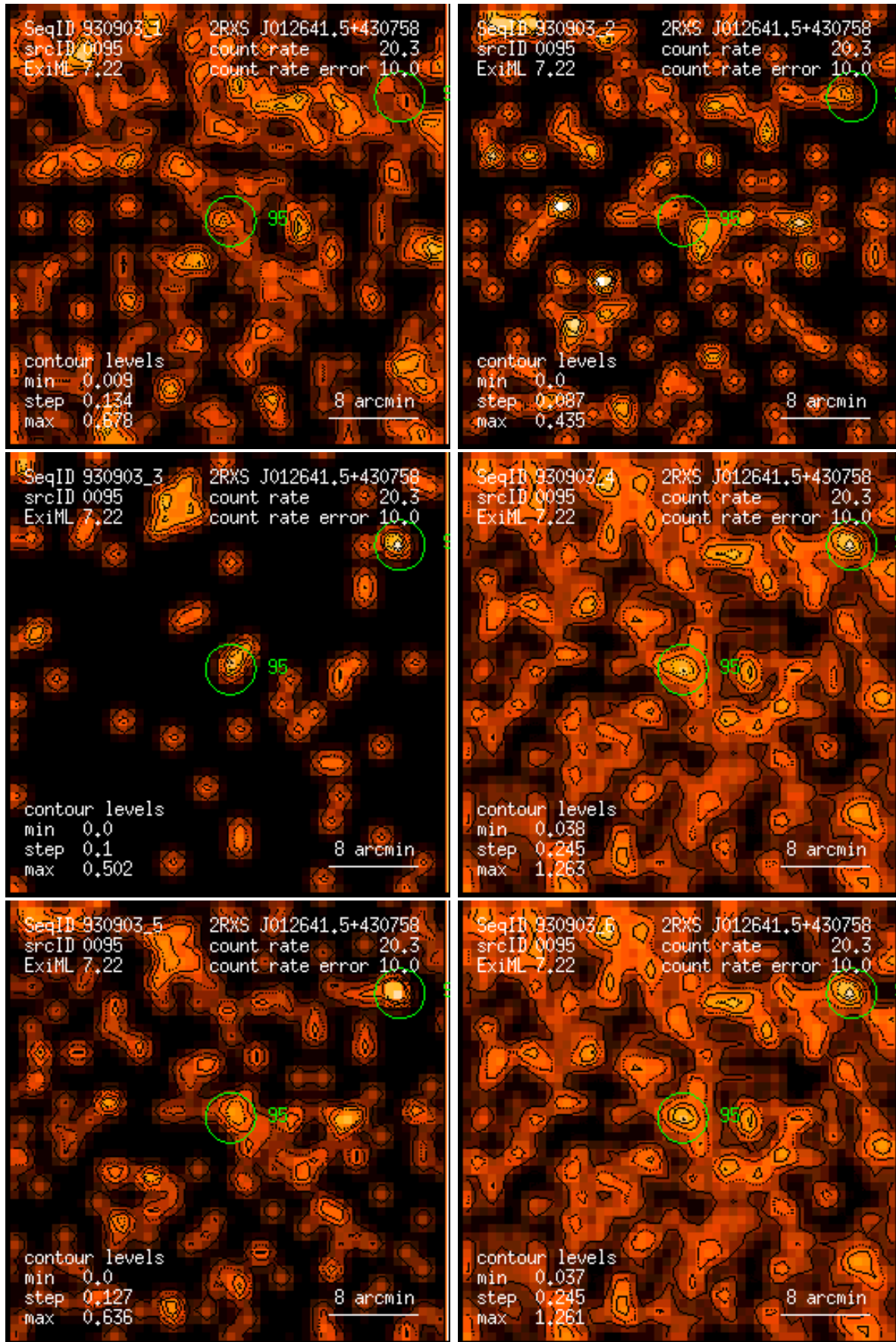
Figure 95: RASS 930903: detection 0095: band rate images, Gaussian filter: (1) PSPC channels 11 – 41, (2) 52 – 90, (3) 91 – 201, (4) 11 – 235, (5) 52 – 201, (6) 11 – 201. Broad band rates in counts/ks. Band rate contour levels in counts/ks/arcmin 2 .
