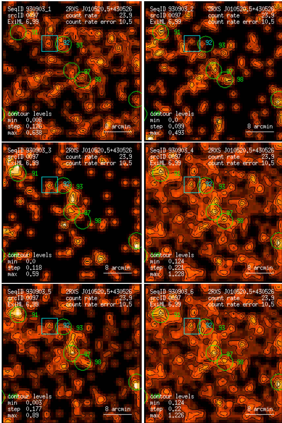
Figure 97: RASS 930903: detection 0097: band rate images, Gaussian filter: (1) PSPC channels 11 – 41, (2) 52 – 90, (3) 91 – 201, (4) 11 – 235, (5) 52 – 201, (6) 11 – 201. Broad band rates in counts/ks. Band rate contour levels in counts/ks/arcmin 2 .
