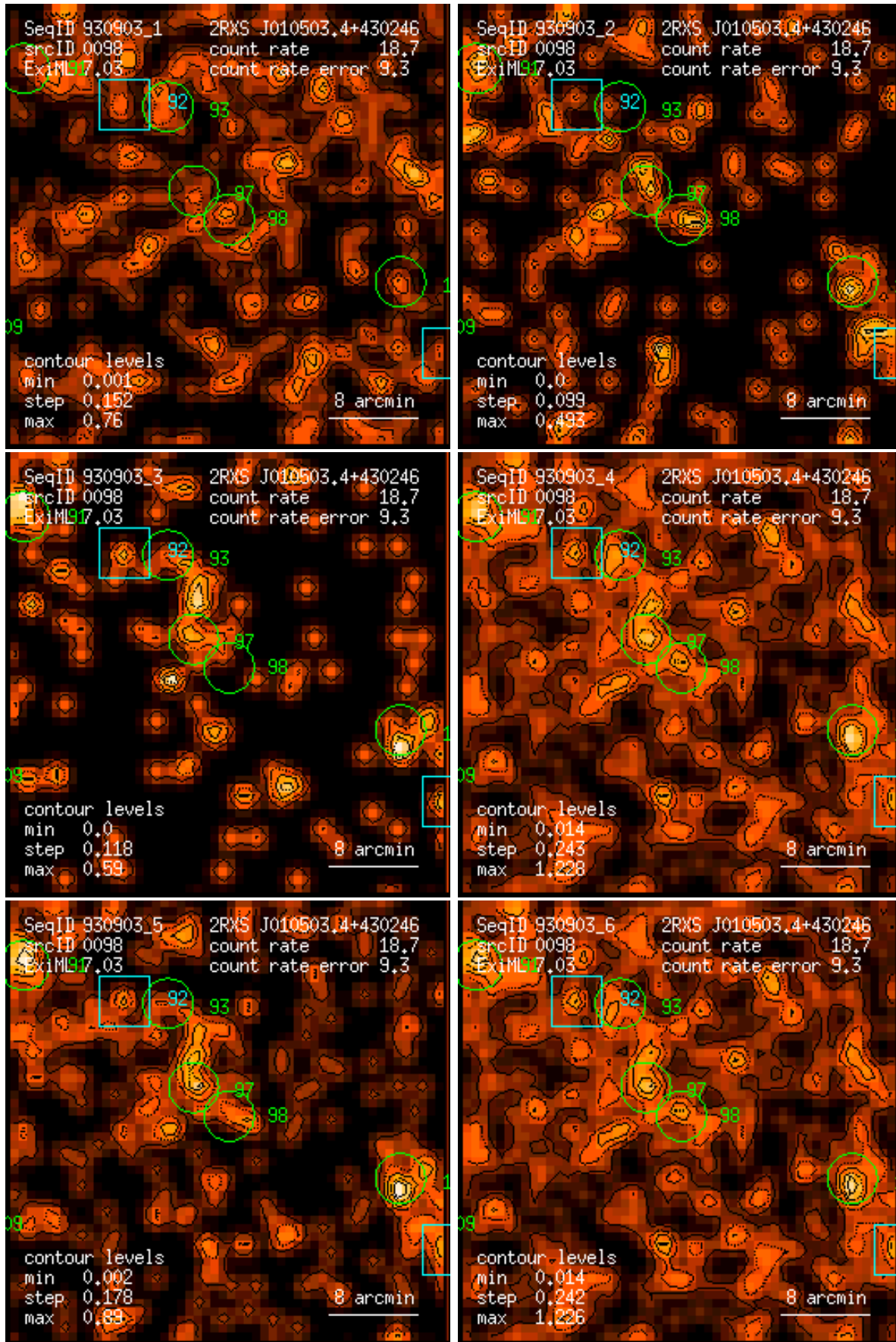
Figure 98: RASS 930903: detection 0098: band rate images, Gaussian filter: (1) PSPC channels 11 – 41, (2) 52 – 90, (3) 91 – 201, (4) 11 – 235, (5) 52 – 201, (6) 11 – 201. Broad band rates in counts/ks. Band rate contour levels in counts/ks/arcmin 2 .
