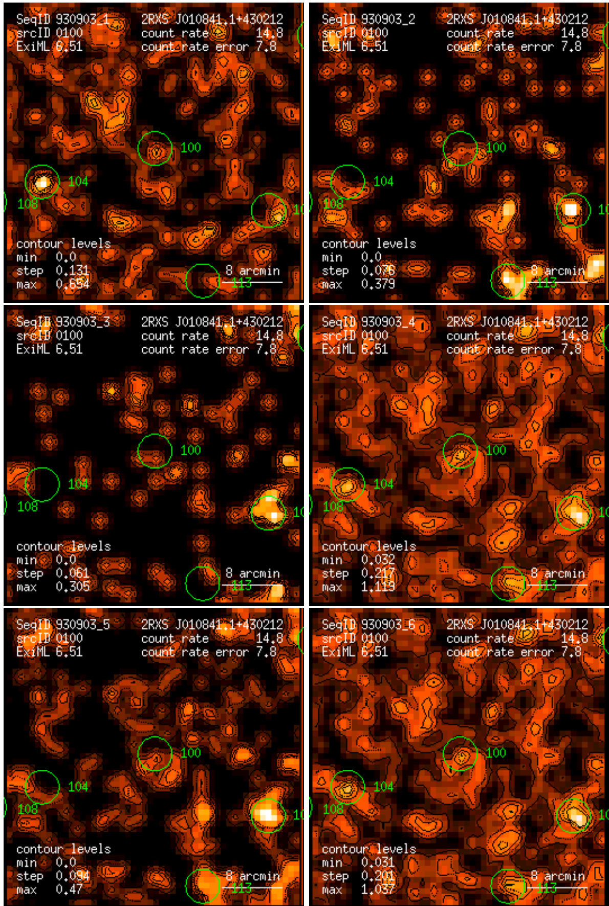
Figure 100: RASS 930903: detection 0100: band rate images, Gaussian filter: (1) PSPC channels 11 – 41, (2) 52 – 90, (3) 91 – 201, (4) 11 – 235, (5) 52 – 201, (6) 11 – 201. Broad band rates in counts/ks. Band rate contour levels in counts/ks/arcmin 2 .
