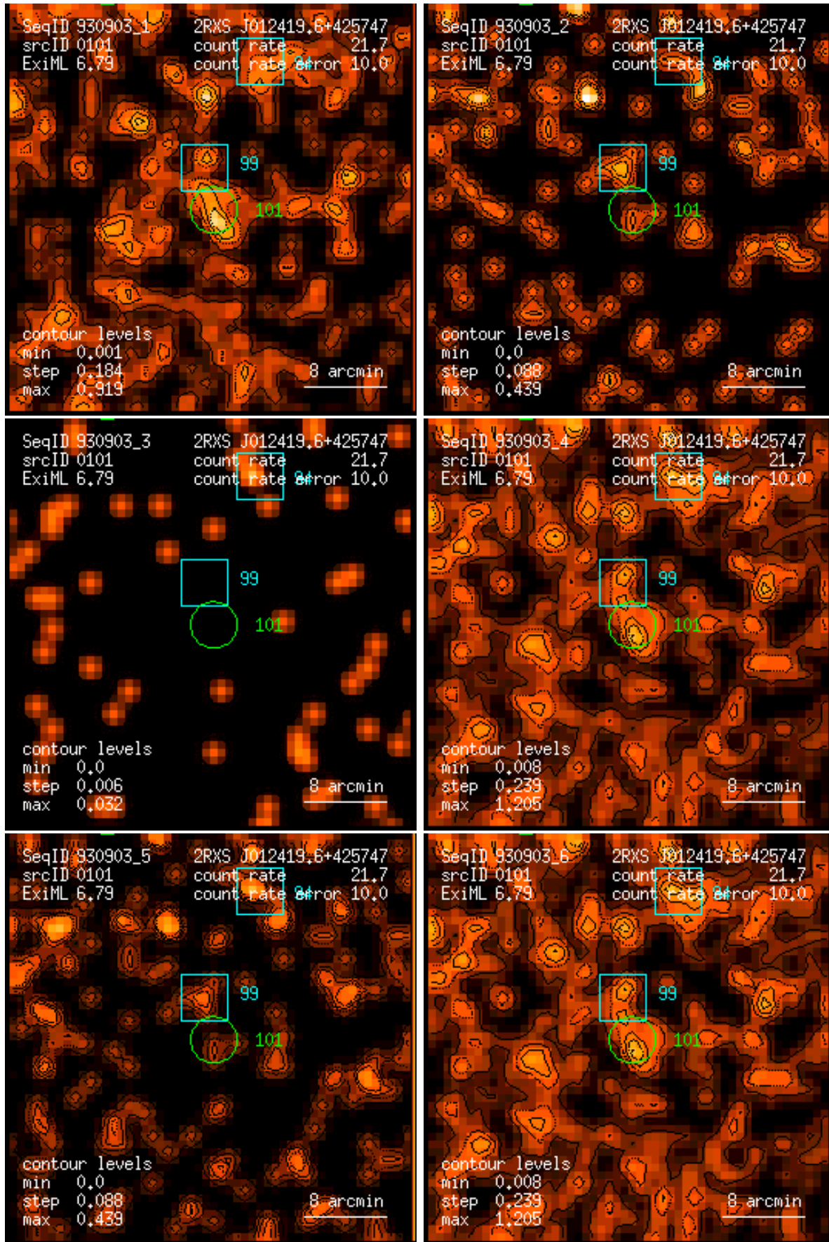
Figure 101: RASS 930903: detection 0101: band rate images, Gaussian filter: (1) PSPC channels 11 – 41, (2) 52 – 90, (3) 91 – 201, (4) 11 – 235, (5) 52 – 201, (6) 11 – 201. Broad band rates in counts/ks. Band rate contour levels in counts/ks/arcmin 2 .
