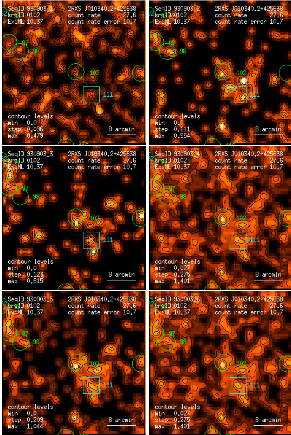
Figure 102: RASS 930903: detection 0102: band rate images, Gaussian filter: (1) PSPC channels 11 – 41, (2) 52 – 90, (3) 91 – 201, (4) 11 – 235, (5) 52 – 201, (6) 11 – 201. Broad band rates in counts/ks. Band rate contour levels in counts/ks/arcmin 2 .
