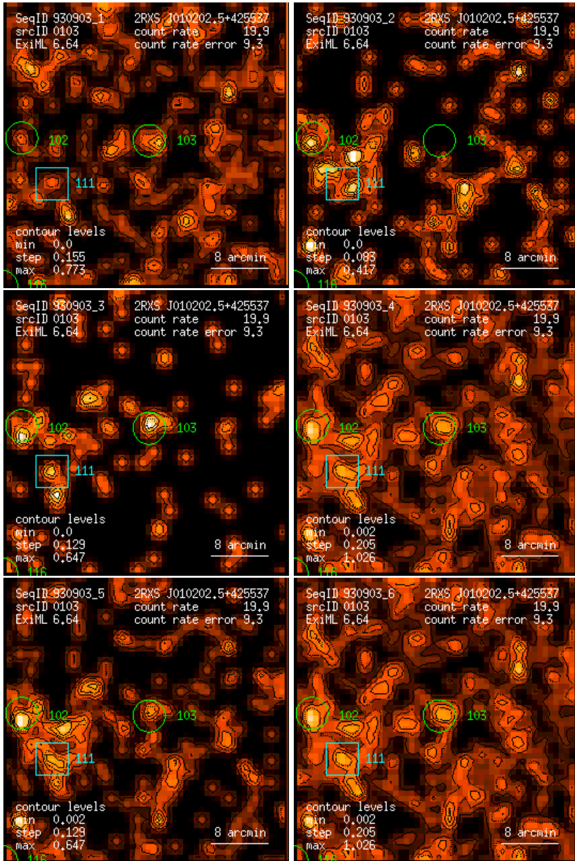
Figure 103: RASS 930903: detection 0103: band rate images, Gaussian filter: (1) PSPC channels 11 – 41, (2) 52 – 90, (3) 91 – 201, (4) 11 – 235, (5) 52 – 201, (6) 11 – 201. Broad band rates in counts/ks. Band rate contour levels in counts/ks/arcmin 2 .
