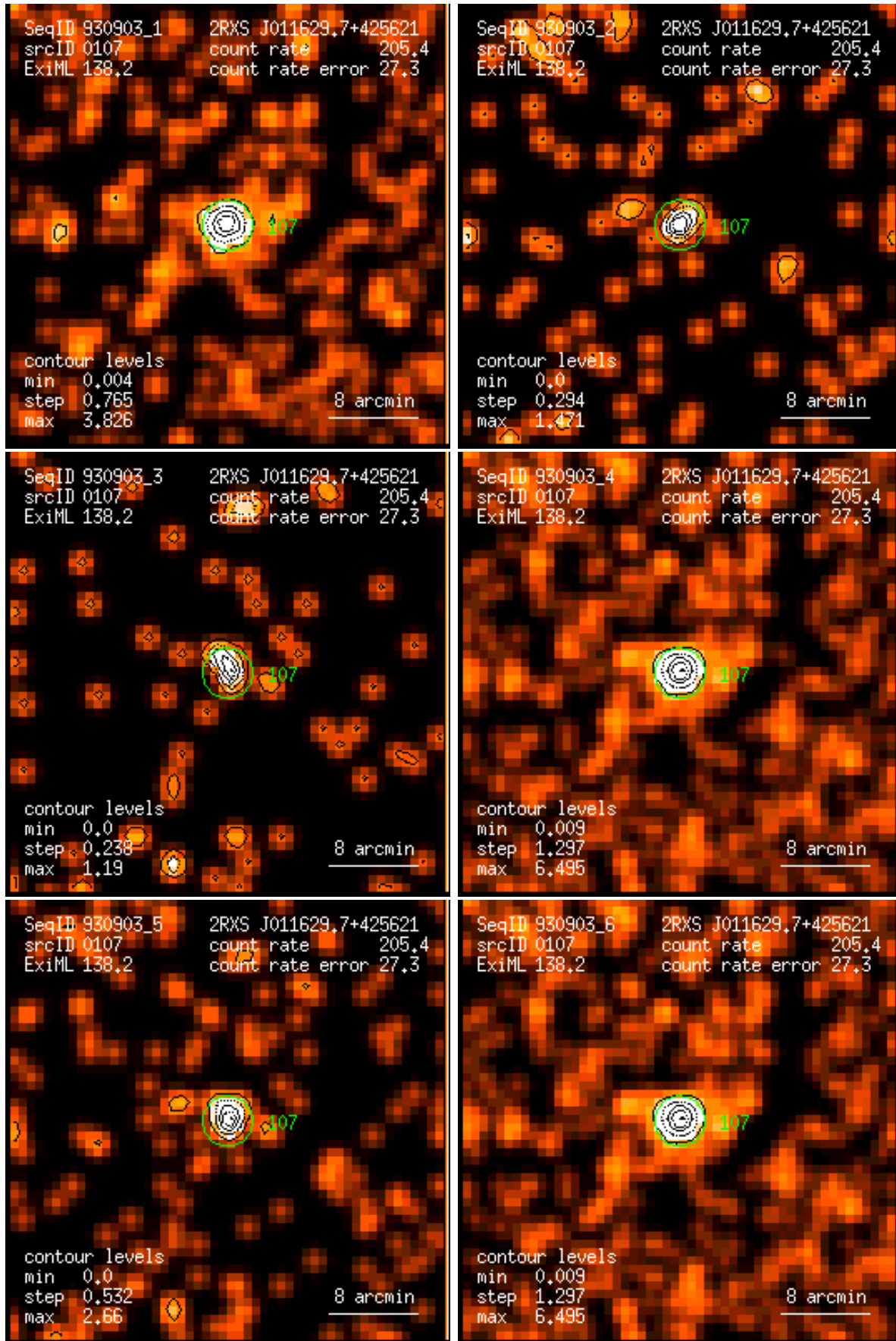
Figure 107: RASS 930903: detection 0107: band rate images, Gaussian filter: (1) PSPC channels 11 – 41, (2) 52 – 90, (3) 91 – 201, (4) 11 – 235, (5) 52 – 201, (6) 11 – 201. Broad band rates in counts/ks. Band rate contour levels in counts/ks/arcmin 2 .
