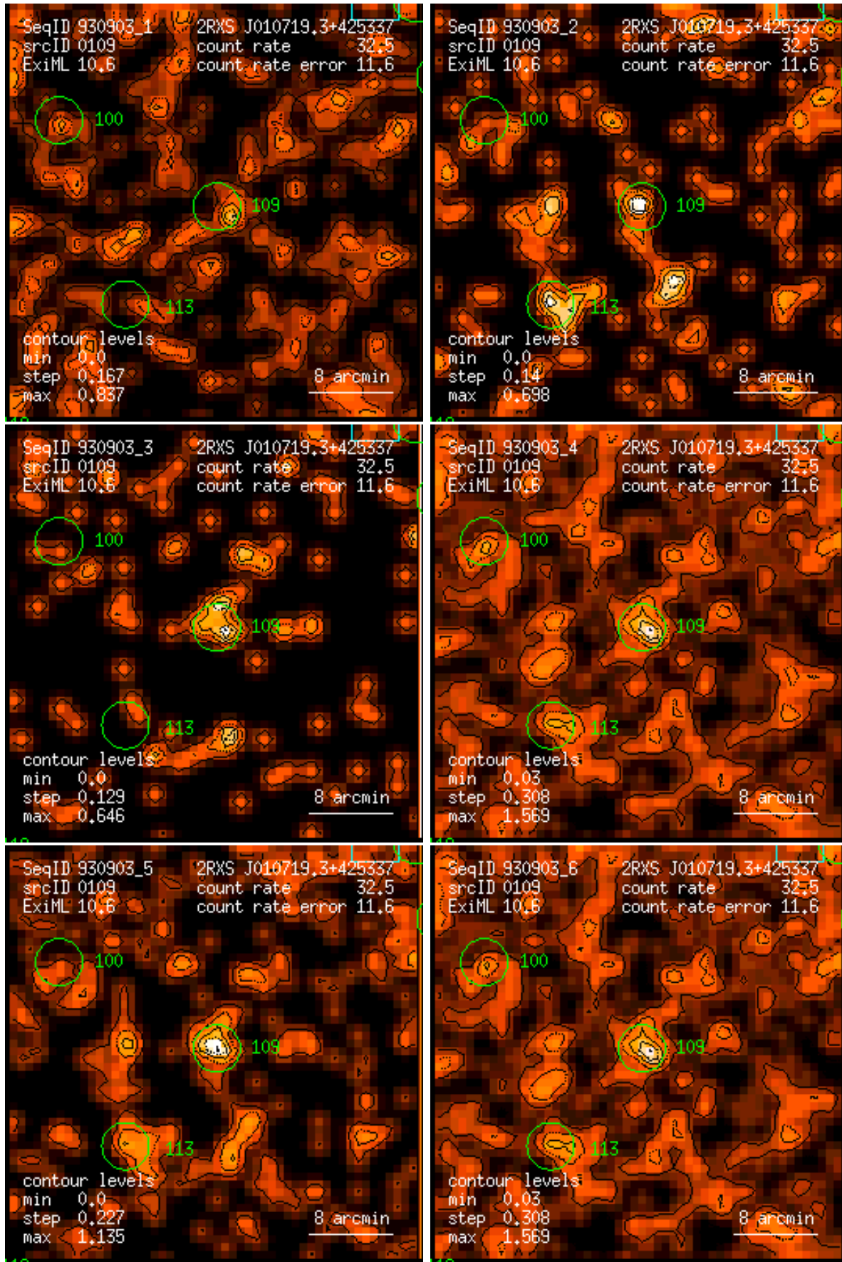
Figure 109: RASS 930903: detection 0109: band rate images, Gaussian filter: (1) PSPC channels 11 – 41, (2) 52 – 90, (3) 91 – 201, (4) 11 – 235, (5) 52 – 201, (6) 11 – 201. Broad band rates in counts/ks. Band rate contour levels in counts/ks/arcmin 2 .
