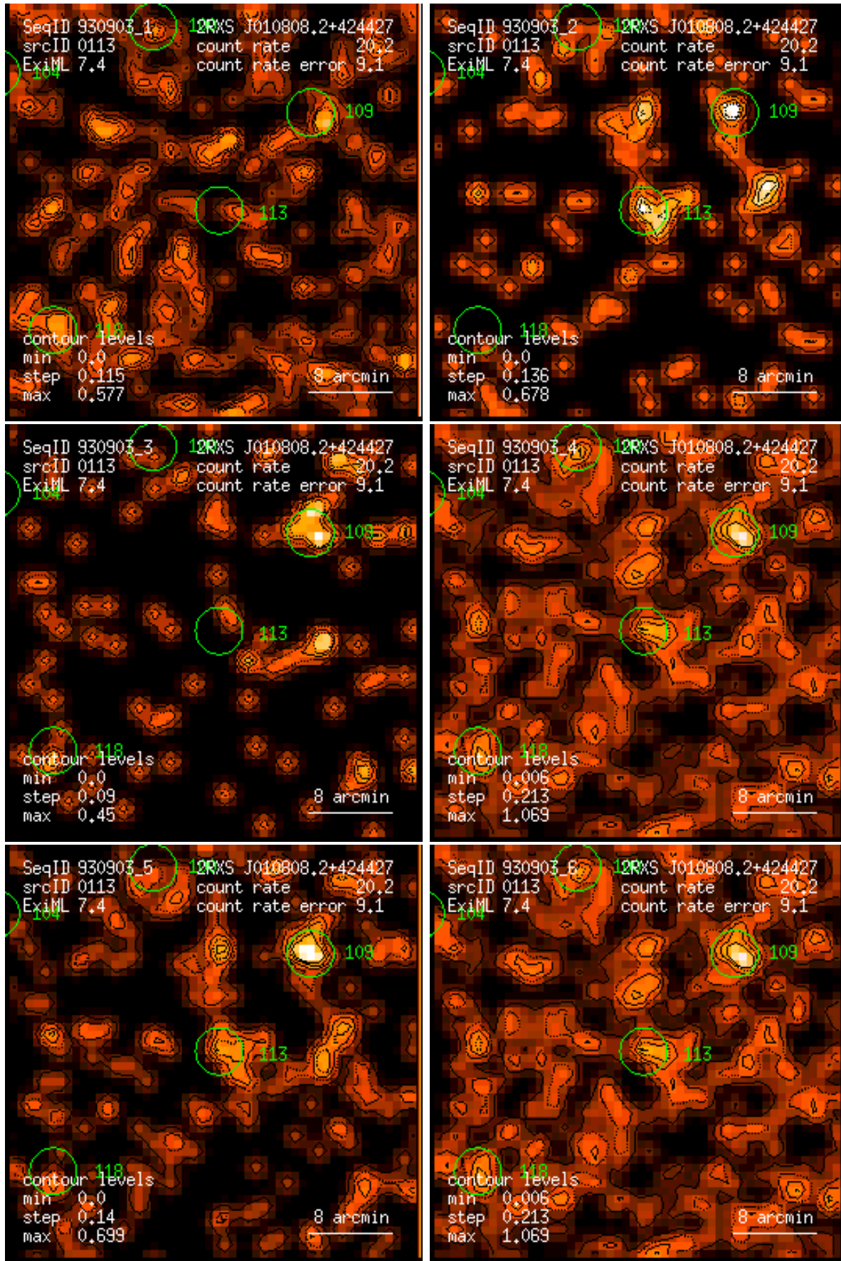
Figure 113: RASS 930903: detection 0113: band rate images, Gaussian filter: (1) PSPC channels 11 – 41, (2) 52 – 90, (3) 91 – 201, (4) 11 – 235, (5) 52 – 201, (6) 11 – 201. Broad band rates in counts/ks. Band rate contour levels in counts/ks/arcmin 2 .
