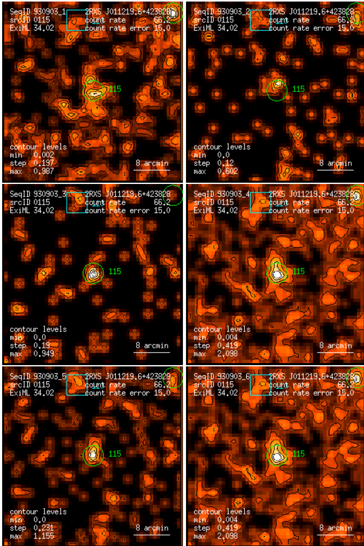
Figure 115: RASS 930903: detection 0115: band rate images, Gaussian filter: (1) PSPC channels 11 – 41, (2) 52 – 90, (3) 91 – 201, (4) 11 – 235, (5) 52 – 201, (6) 11 – 201. Broad band rates in counts/ks. Band rate contour levels in counts/ks/arcmin 2 .
