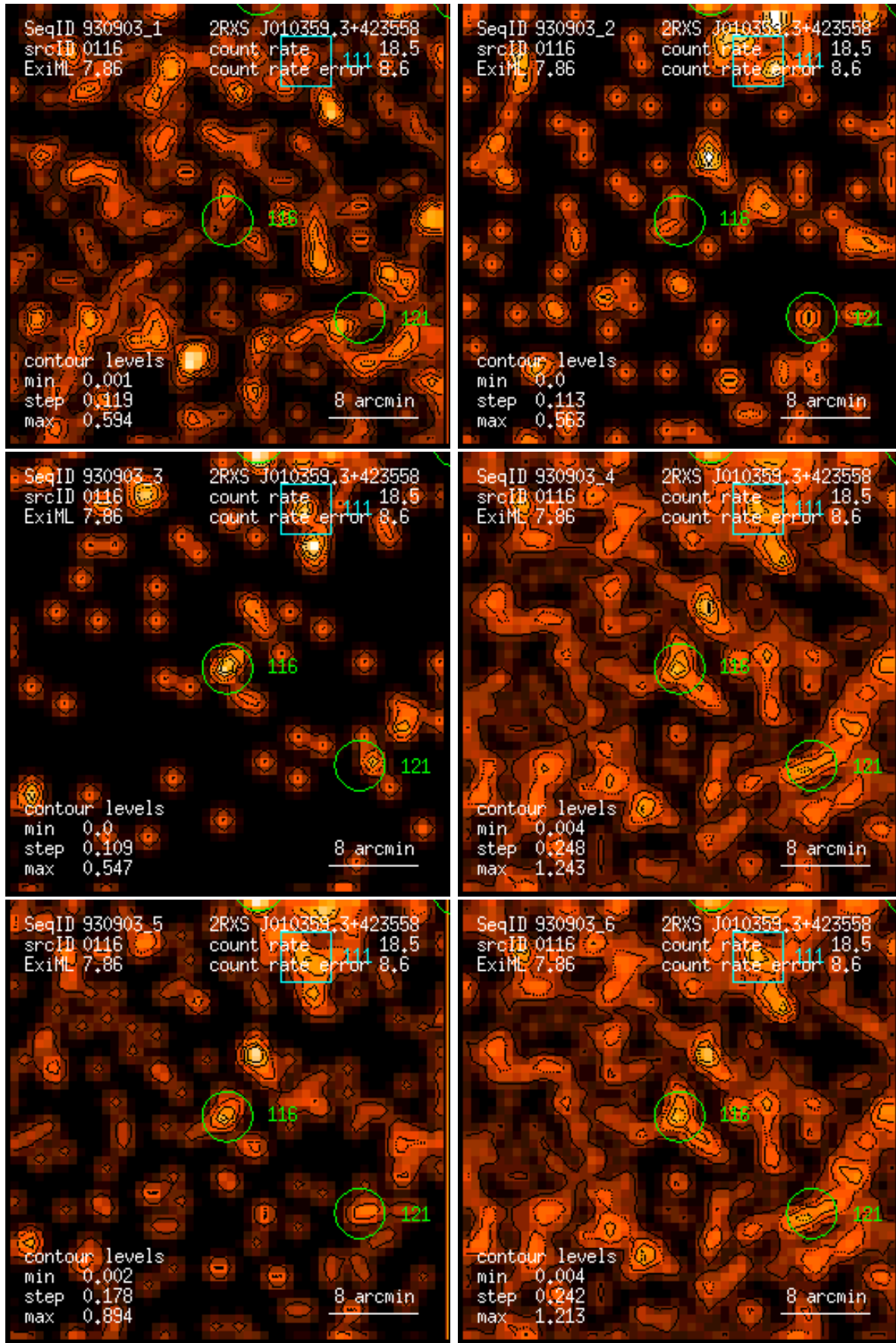
Figure 116: RASS 930903: detection 0116: band rate images, Gaussian filter: (1) PSPC channels 11 – 41, (2) 52 – 90, (3) 91 – 201, (4) 11 – 235, (5) 52 – 201, (6) 11 – 201. Broad band rates in counts/ks. Band rate contour levels in counts/ks/arcmin 2 .
