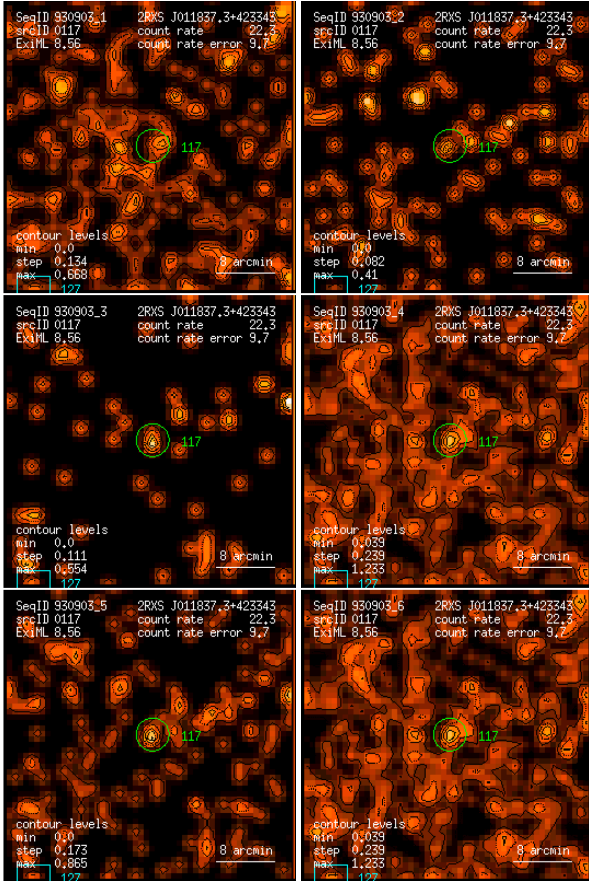
Figure 117: RASS 930903: detection 0117: band rate images, Gaussian filter: (1) PSPC channels 11 – 41, (2) 52 – 90, (3) 91 – 201, (4) 11 – 235, (5) 52 – 201, (6) 11 – 201. Broad band rates in counts/ks. Band rate contour levels in counts/ks/arcmin 2 .
