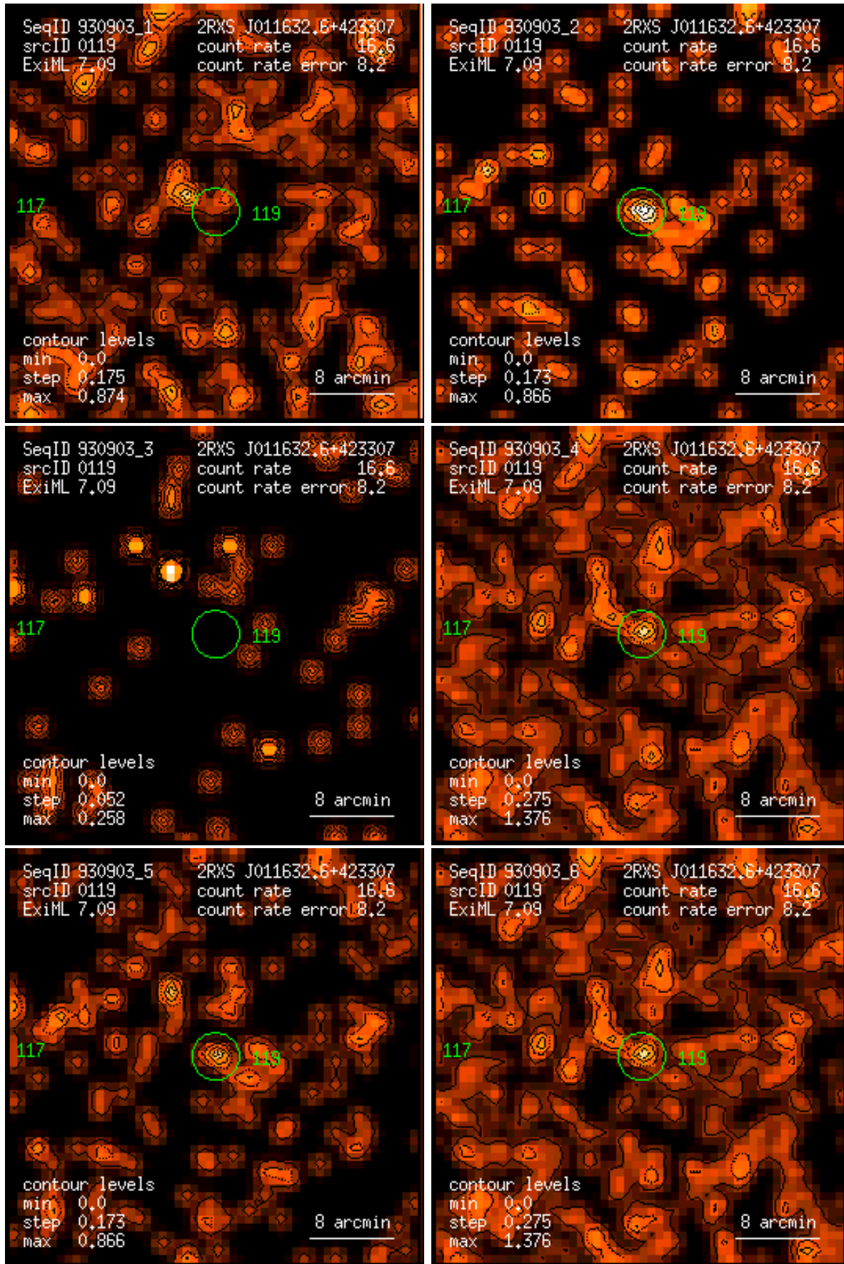
Figure 119: RASS 930903: detection 0119: band rate images, Gaussian filter: (1) PSPC channels 11 – 41, (2) 52 – 90, (3) 91 – 201, (4) 11 – 235, (5) 52 – 201, (6) 11 – 201. Broad band rates in counts/ks. Band rate contour levels in counts/ks/arcmin 2 .
