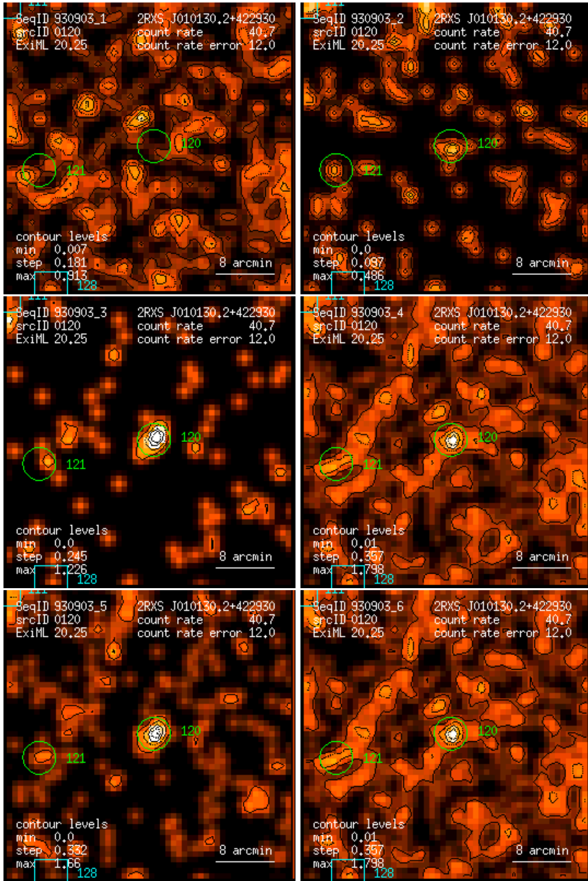
Figure 120: RASS 930903: detection 0120: band rate images, Gaussian filter: (1) PSPC channels 11 – 41, (2) 52 – 90, (3) 91 – 201, (4) 11 – 235, (5) 52 – 201, (6) 11 – 201. Broad band rates in counts/ks. Band rate contour levels in counts/ks/arcmin 2 .
