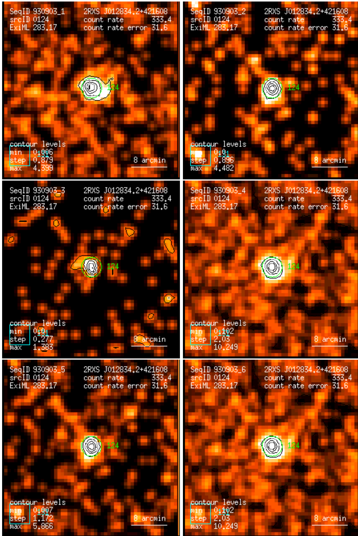
Figure 124: RASS 930903: detection 0124: band rate images, Gaussian filter: (1) PSPC channels 11 – 41, (2) 52 – 90, (3) 91 – 201, (4) 11 – 235, (5) 52 – 201, (6) 11 – 201. Broad band rates in counts/ks. Band rate contour levels in counts/ks/arcmin 2 .
