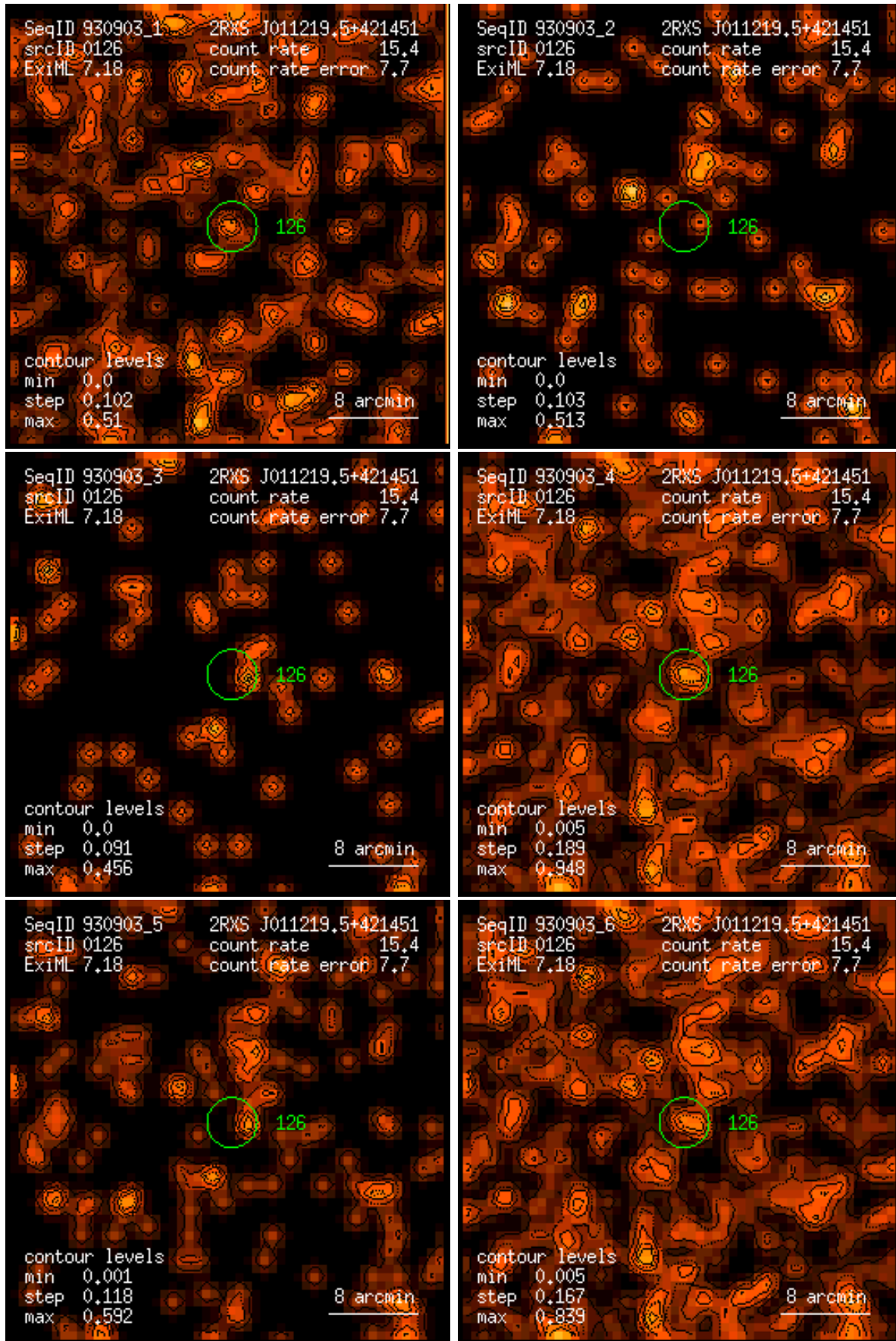
Figure 126: RASS 930903: detection 0126: band rate images, Gaussian filter: (1) PSPC channels 11 – 41, (2) 52 – 90, (3) 91 – 201, (4) 11 – 235, (5) 52 – 201, (6) 11 – 201. Broad band rates in counts/ks. Band rate contour levels in counts/ks/arcmin 2 .
