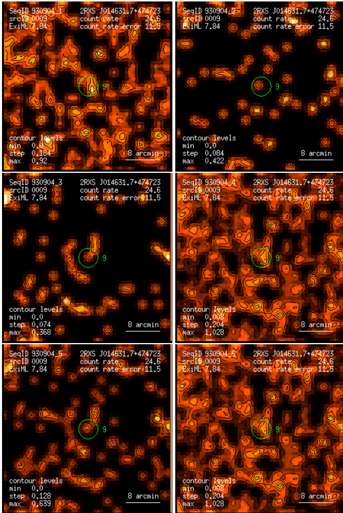
Figure 9: RASS 930904: detection 0009: band rate images, Gaussian filter: (1) PSPC channels 11 – 41, (2) 52 – 90, (3) 91 – 201, (4) 11 – 235, (5) 52 – 201, (6) 11 – 201. Broad band rates in counts/ks. Band rate contour levels in counts/ks/arcmin 2 .
