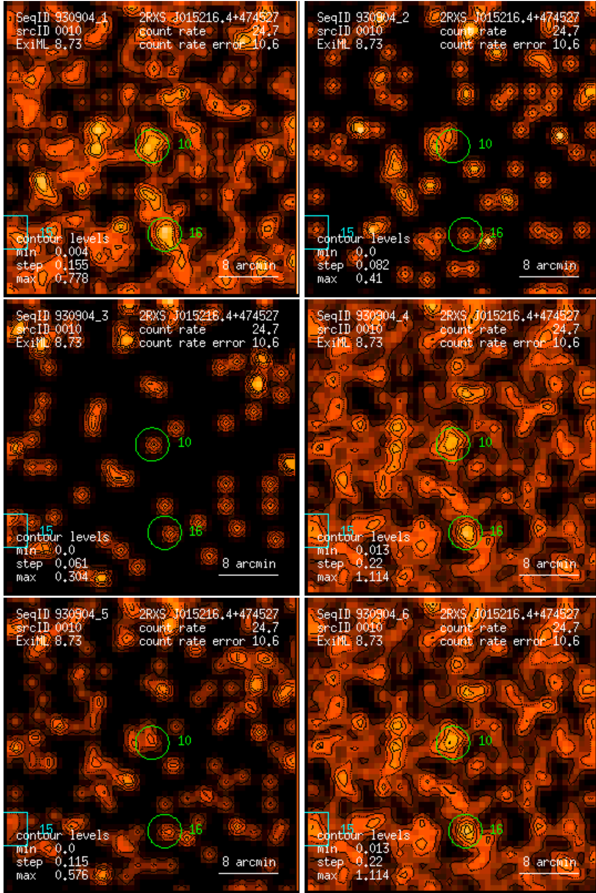
Figure 10: RASS 930904: detection 0010: band rate images, Gaussian filter: (1) PSPC channels 11 – 41, (2) 52 – 90, (3) 91 – 201, (4) 11 – 235, (5) 52 – 201, (6) 11 – 201. Broad band rates in counts/ks. Band rate contour levels in counts/ks/arcmin 2 .
