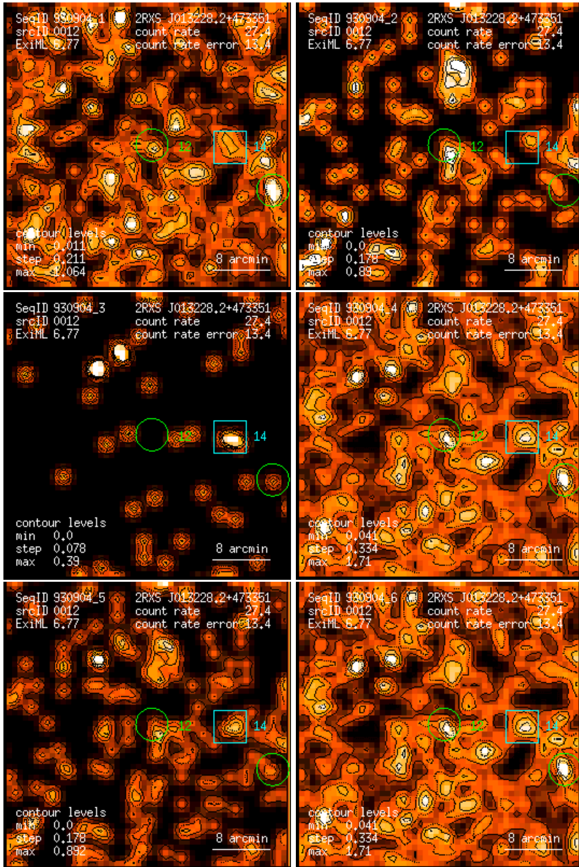
Figure 12: RASS 930904: detection 0012: band rate images, Gaussian filter: (1) PSPC channels 11 – 41, (2) 52 – 90, (3) 91 – 201, (4) 11 – 235, (5) 52 – 201, (6) 11 – 201. Broad band rates in counts/ks. Band rate contour levels in counts/ks/arcmin 2 .
