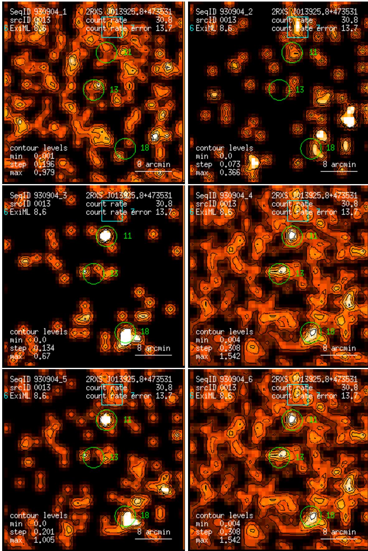
Figure 13: RASS 930904: detection 0013: band rate images, Gaussian filter: (1) PSPC channels 11 – 41, (2) 52 – 90, (3) 91 – 201, (4) 11 – 235, (5) 52 – 201, (6) 11 – 201. Broad band rates in counts/ks. Band rate contour levels in counts/ks/arcmin 2 .
