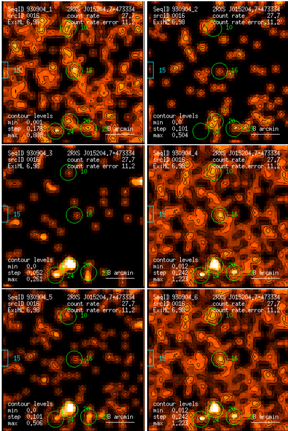
Figure 16: RASS 930904: detection 0016: band rate images, Gaussian filter: (1) PSPC channels 11 – 41, (2) 52 – 90, (3) 91 – 201, (4) 11 – 235, (5) 52 – 201, (6) 11 – 201. Broad band rates in counts/ks. Band rate contour levels in counts/ks/arcmin 2 .
