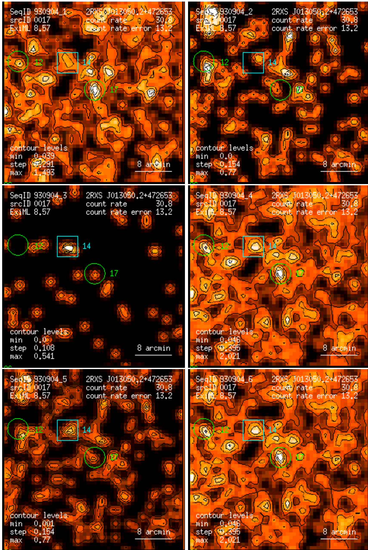
Figure 17: RASS 930904: detection 0017: band rate images, Gaussian filter: (1) PSPC channels 11 – 41, (2) 52 – 90, (3) 91 – 201, (4) 11 – 235, (5) 52 – 201, (6) 11 – 201. Broad band rates in counts/ks. Band rate contour levels in counts/ks/arcmin 2 .
