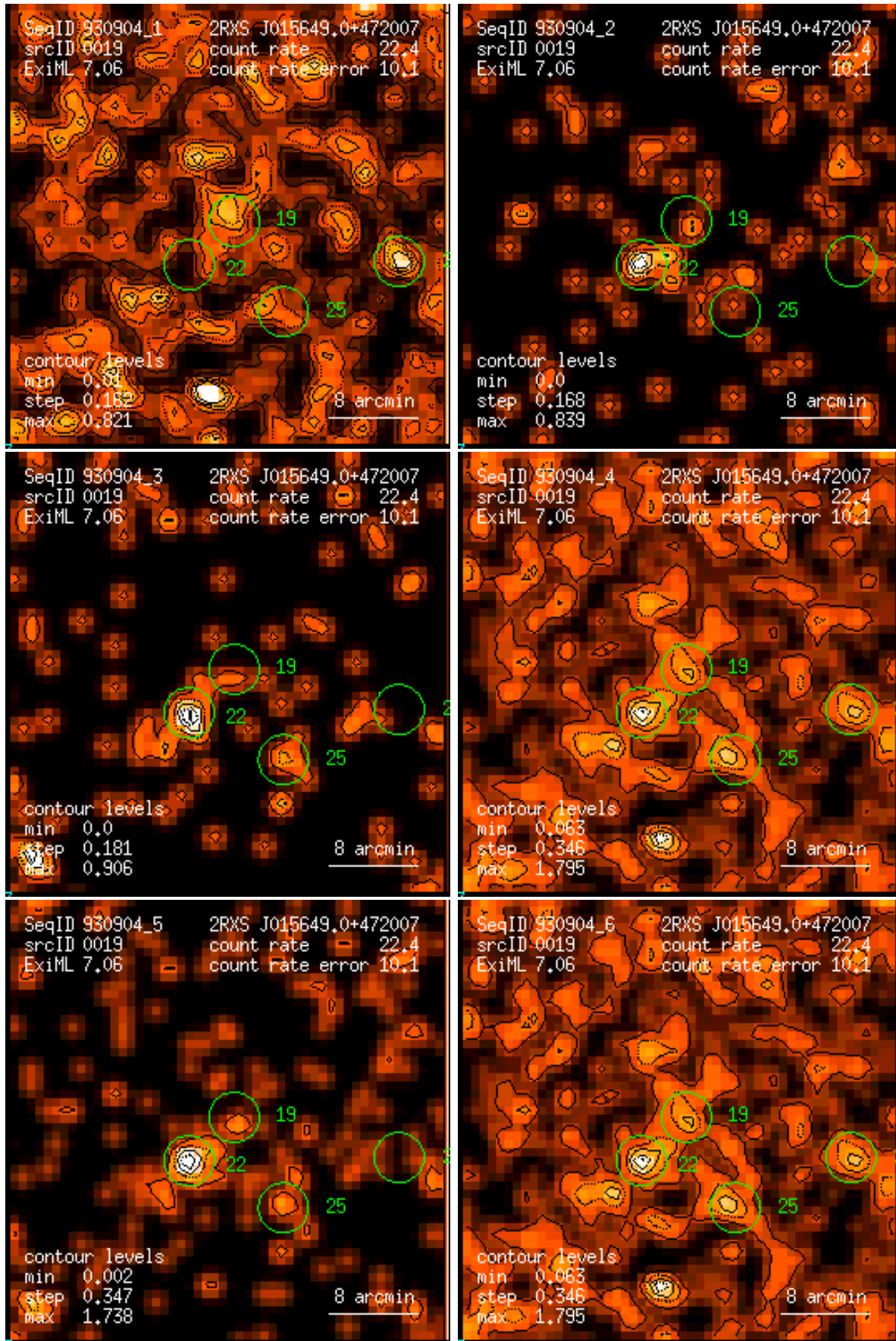
Figure 19: RASS 930904: detection 0019: band rate images, Gaussian filter: (1) PSPC channels 11 – 41, (2) 52 – 90, (3) 91 – 201, (4) 11 – 235, (5) 52 – 201, (6) 11 – 201. Broad band rates in counts/ks. Band rate contour levels in counts/ks/arcmin 2 .
