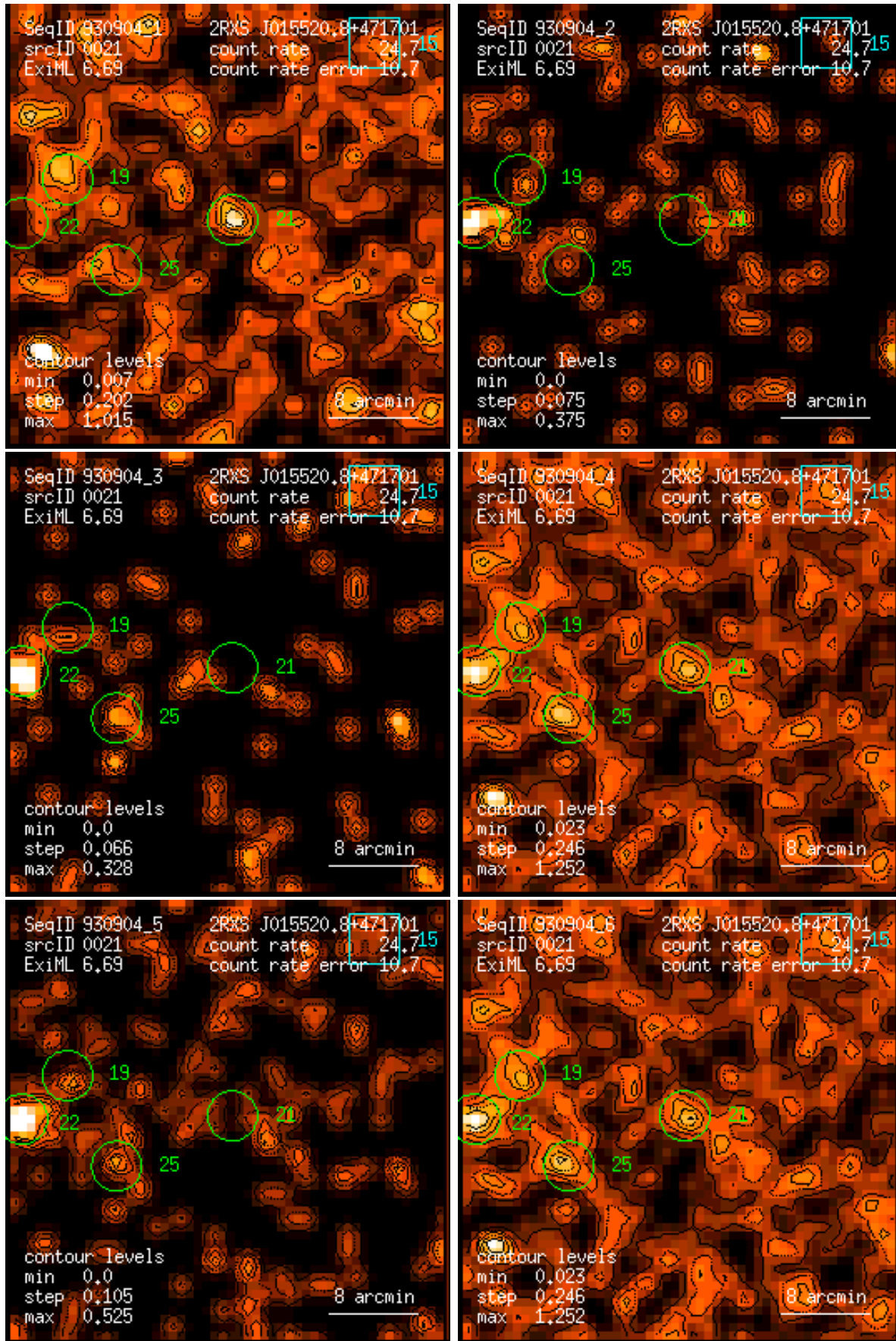
Figure 21: RASS 930904: detection 0021: band rate images, Gaussian filter: (1) PSPC channels 11 – 41, (2) 52 – 90, (3) 91 – 201, (4) 11 – 235, (5) 52 – 201, (6) 11 – 201. Broad band rates in counts/ks. Band rate contour levels in counts/ks/arcmin 2 .
