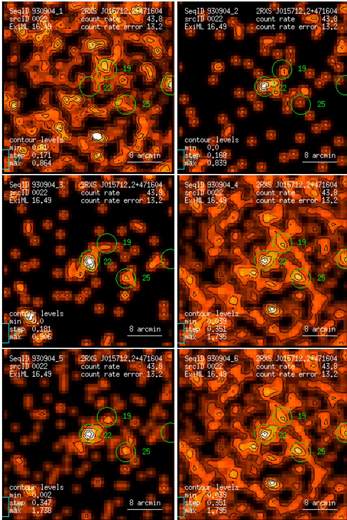
Figure 22: RASS 930904: detection 0022: band rate images, Gaussian filter: (1) PSPC channels 11 – 41, (2) 52 – 90, (3) 91 – 201, (4) 11 – 235, (5) 52 – 201, (6) 11 – 201. Broad band rates in counts/ks. Band rate contour levels in counts/ks/arcmin 2 .
