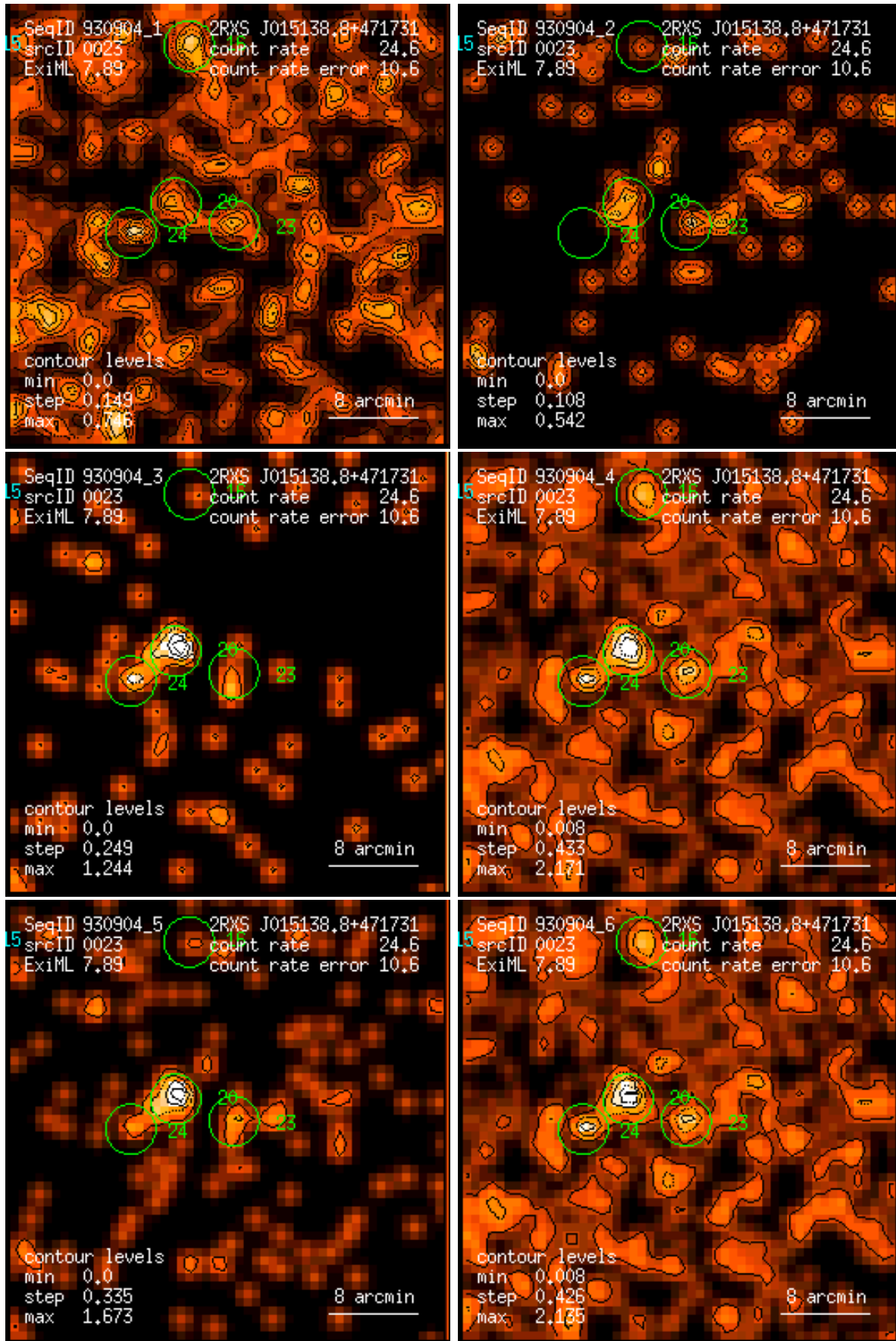
Figure 23: RASS 930904: detection 0023: band rate images, Gaussian filter: (1) PSPC channels 11 – 41, (2) 52 – 90, (3) 91 – 201, (4) 11 – 235, (5) 52 – 201, (6) 11 – 201. Broad band rates in counts/ks. Band rate contour levels in counts/ks/arcmin 2 .
