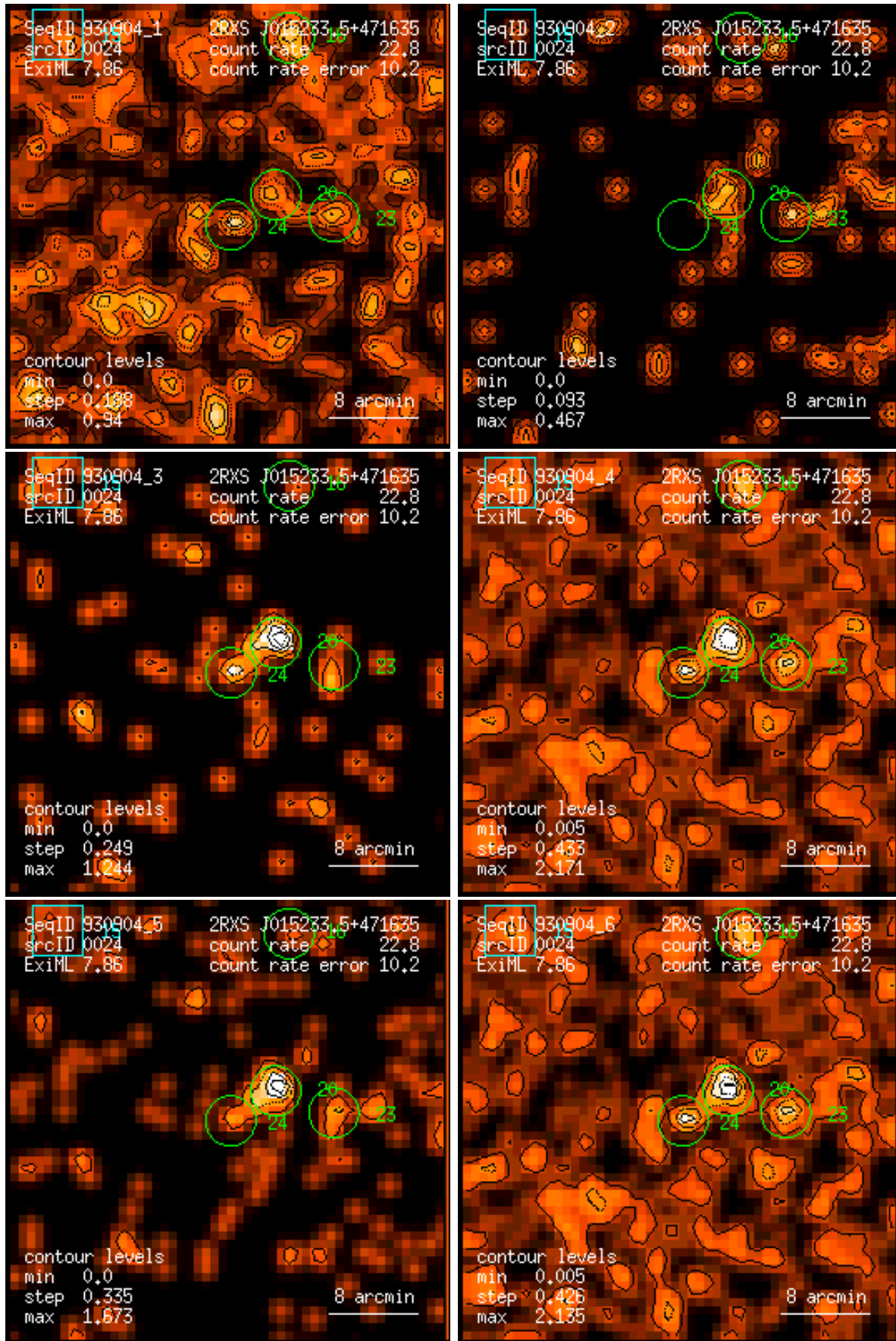
Figure 24: RASS 930904: detection 0024: band rate images, Gaussian filter: (1) PSPC channels 11 – 41, (2) 52 – 90, (3) 91 – 201, (4) 11 – 235, (5) 52 – 201, (6) 11 – 201. Broad band rates in counts/ks. Band rate contour levels in counts/ks/arcmin 2 .
