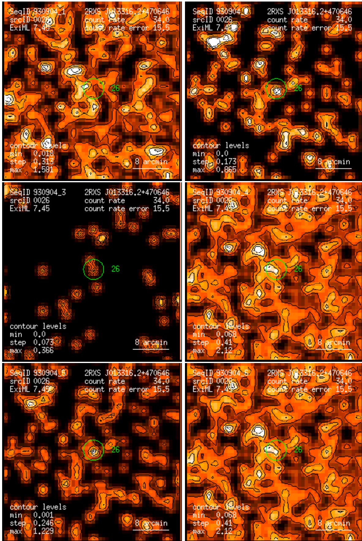
Figure 26: RASS 930904: detection 0026: band rate images, Gaussian filter: (1) PSPC channels 11 – 41, (2) 52 – 90, (3) 91 – 201, (4) 11 – 235, (5) 52 – 201, (6) 11 – 201. Broad band rates in counts/ks. Band rate contour levels in counts/ks/arcmin 2 .
