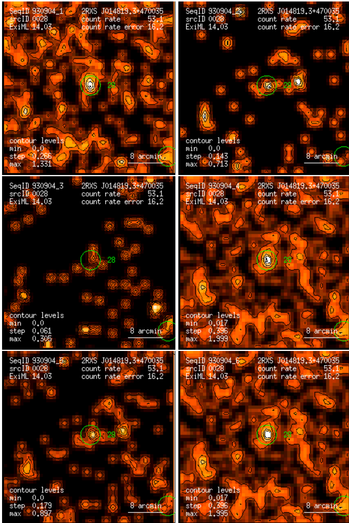
Figure 28: RASS 930904: detection 0028: band rate images, Gaussian filter: (1) PSPC channels 11 – 41, (2) 52 – 90, (3) 91 – 201, (4) 11 – 235, (5) 52 – 201, (6) 11 – 201. Broad band rates in counts/ks. Band rate contour levels in counts/ks/arcmin 2 .
