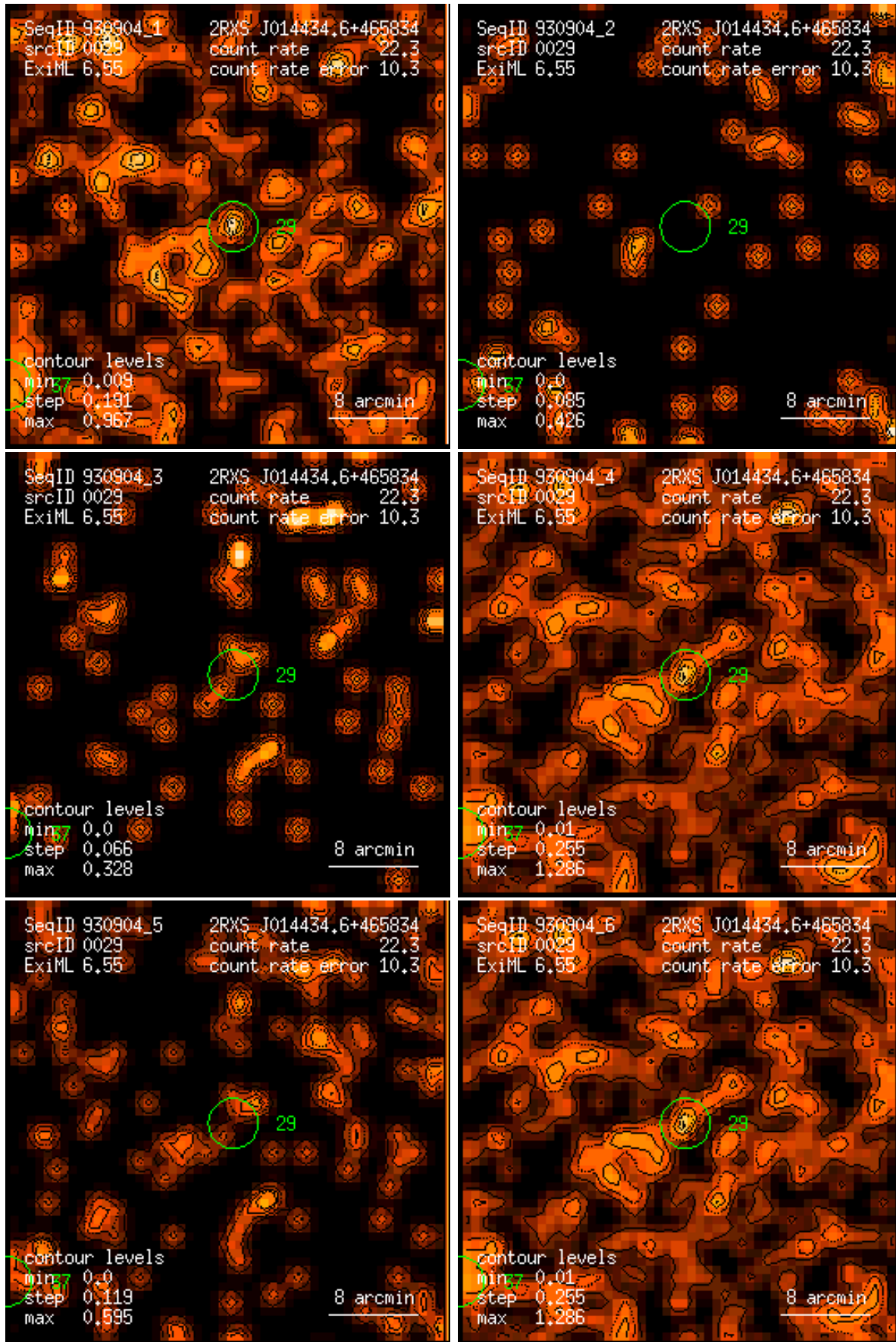
Figure 29: RASS 930904: detection 0029: band rate images, Gaussian filter: (1) PSPC channels 11 – 41, (2) 52 – 90, (3) 91 – 201, (4) 11 – 235, (5) 52 – 201, (6) 11 – 201. Broad band rates in counts/ks. Band rate contour levels in counts/ks/arcmin 2 .
