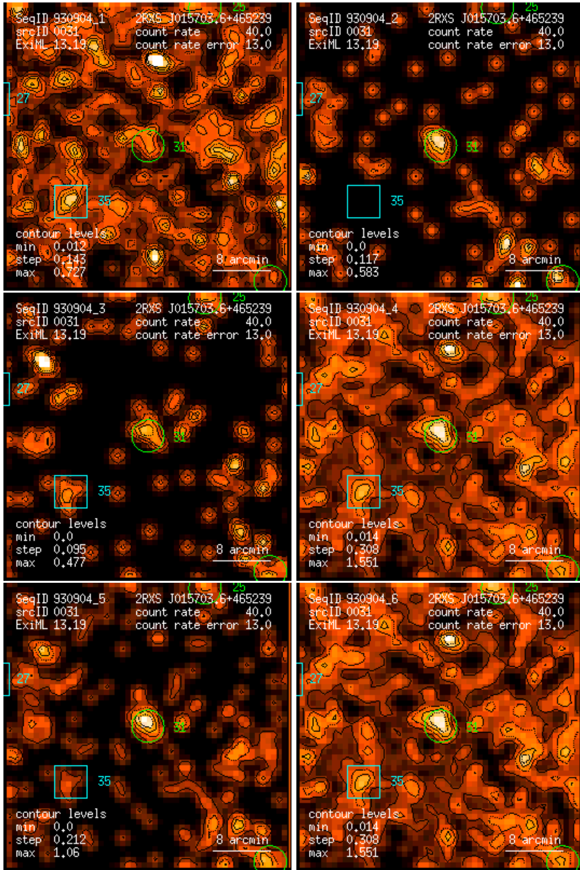
Figure 31: RASS 930904: detection 0031: band rate images, Gaussian filter: (1) PSPC channels 11 – 41, (2) 52 – 90, (3) 91 – 201, (4) 11 – 235, (5) 52 – 201, (6) 11 – 201. Broad band rates in counts/ks. Band rate contour levels in counts/ks/arcmin 2 .
