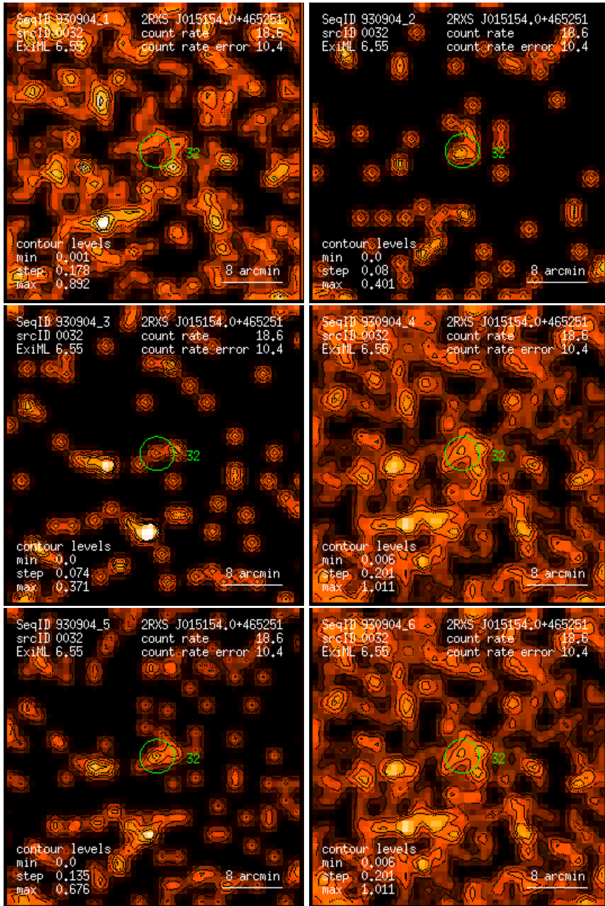
Figure 32: RASS 930904: detection 0032: band rate images, Gaussian filter: (1) PSPC channels 11 – 41, (2) 52 – 90, (3) 91 – 201, (4) 11 – 235, (5) 52 – 201, (6) 11 – 201. Broad band rates in counts/ks. Band rate contour levels in counts/ks/arcmin 2 .
