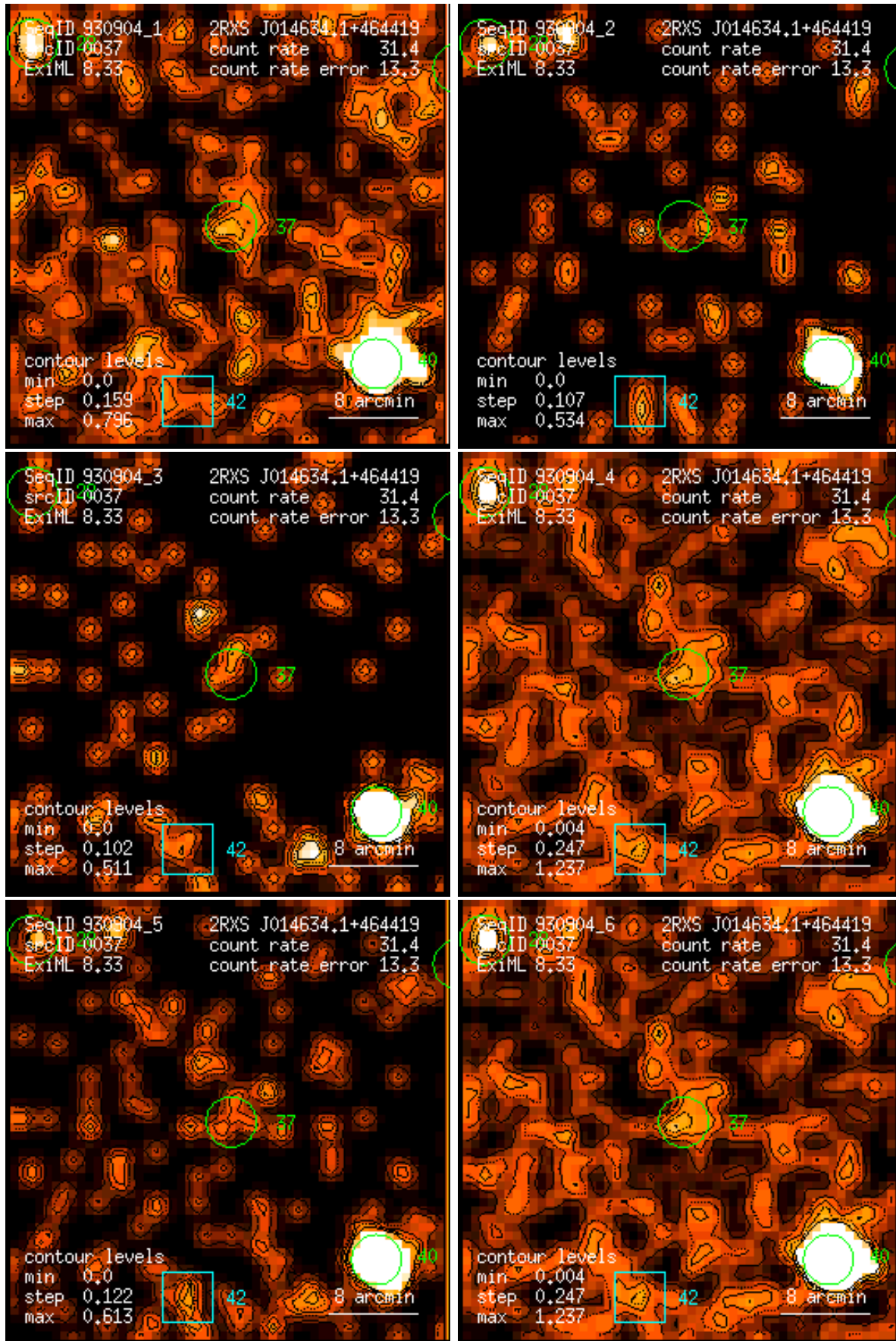
Figure 37: RASS 930904: detection 0037: band rate images, Gaussian filter: (1) PSPC channels 11 – 41, (2) 52 – 90, (3) 91 – 201, (4) 11 – 235, (5) 52 – 201, (6) 11 – 201. Broad band rates in counts/ks. Band rate contour levels in counts/ks/arcmin 2 .
