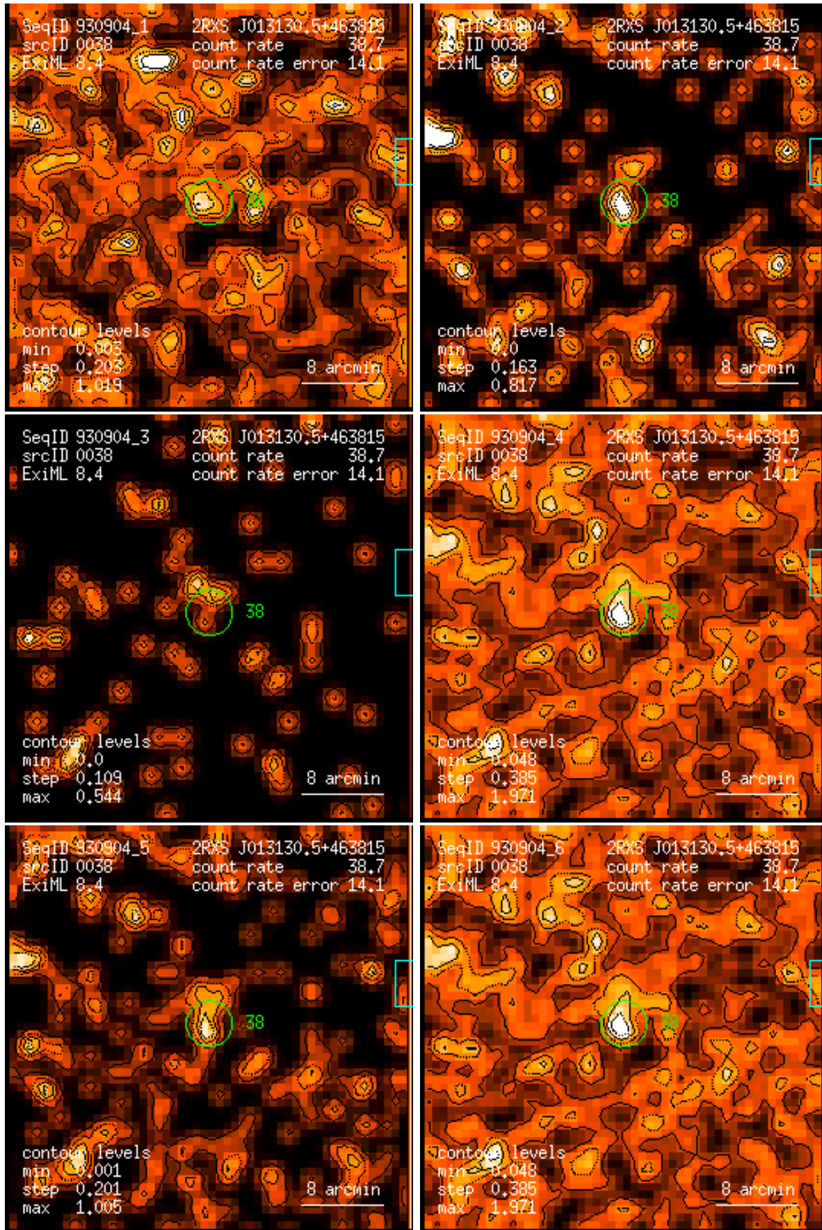
Figure 38: RASS 930904: detection 0038: band rate images, Gaussian filter: (1) PSPC channels 11 – 41, (2) 52 – 90, (3) 91 – 201, (4) 11 – 235, (5) 52 – 201, (6) 11 – 201. Broad band rates in counts/ks. Band rate contour levels in counts/ks/arcmin 2 .
