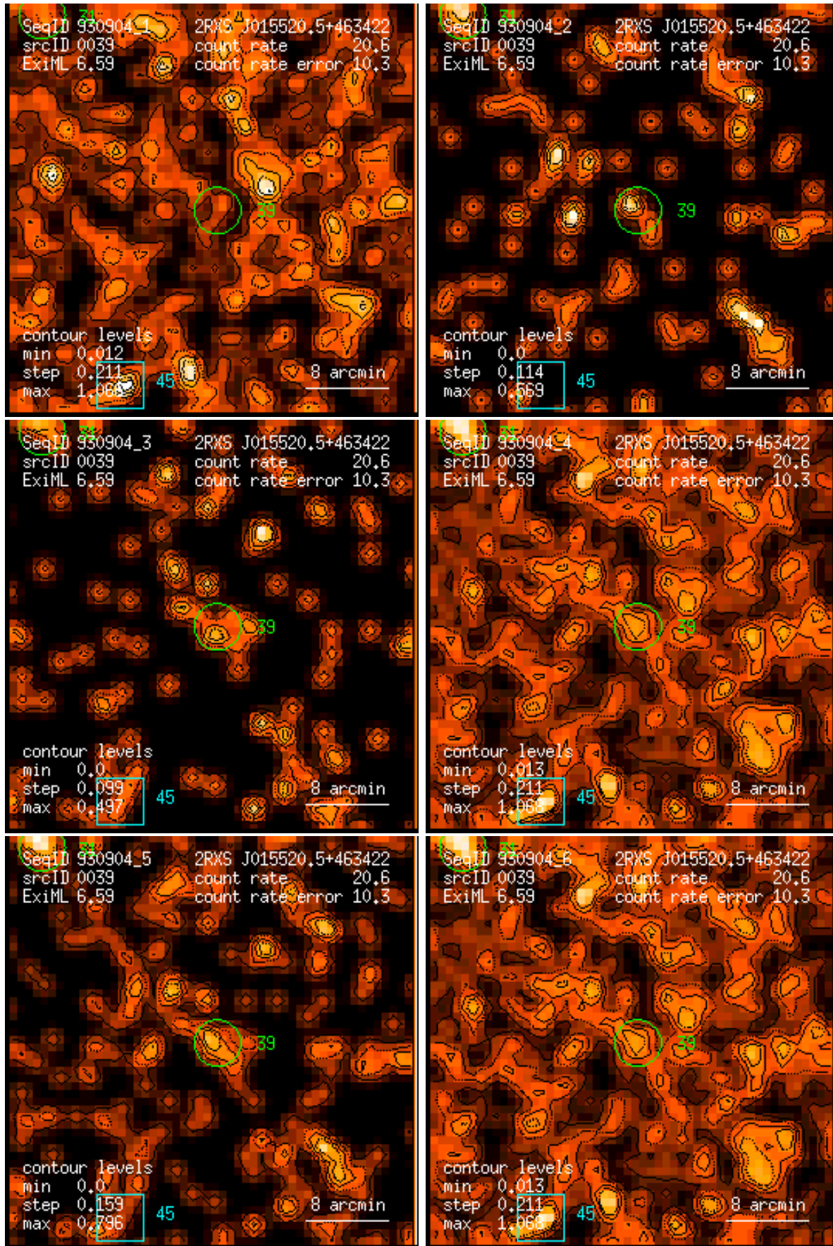
Figure 39: RASS 930904: detection 0039: band rate images, Gaussian filter: (1) PSPC channels 11 – 41, (2) 52 – 90, (3) 91 – 201, (4) 11 – 235, (5) 52 – 201, (6) 11 – 201. Broad band rates in counts/ks. Band rate contour levels in counts/ks/arcmin 2 .
