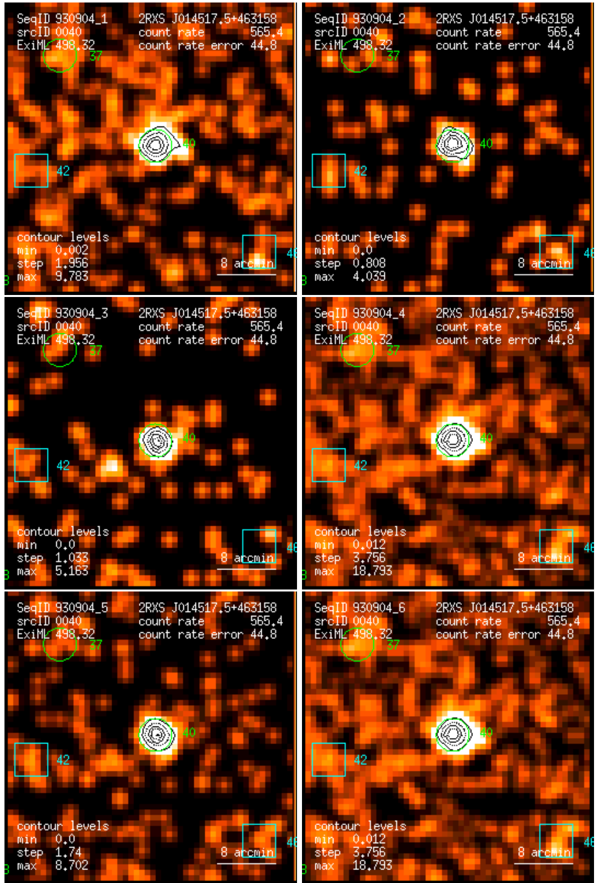
Figure 40: RASS 930904: detection 0040: band rate images, Gaussian filter: (1) PSPC channels 11 – 41, (2) 52 – 90, (3) 91 – 201, (4) 11 – 235, (5) 52 – 201, (6) 11 – 201. Broad band rates in counts/ks. Band rate contour levels in counts/ks/arcmin 2 .
