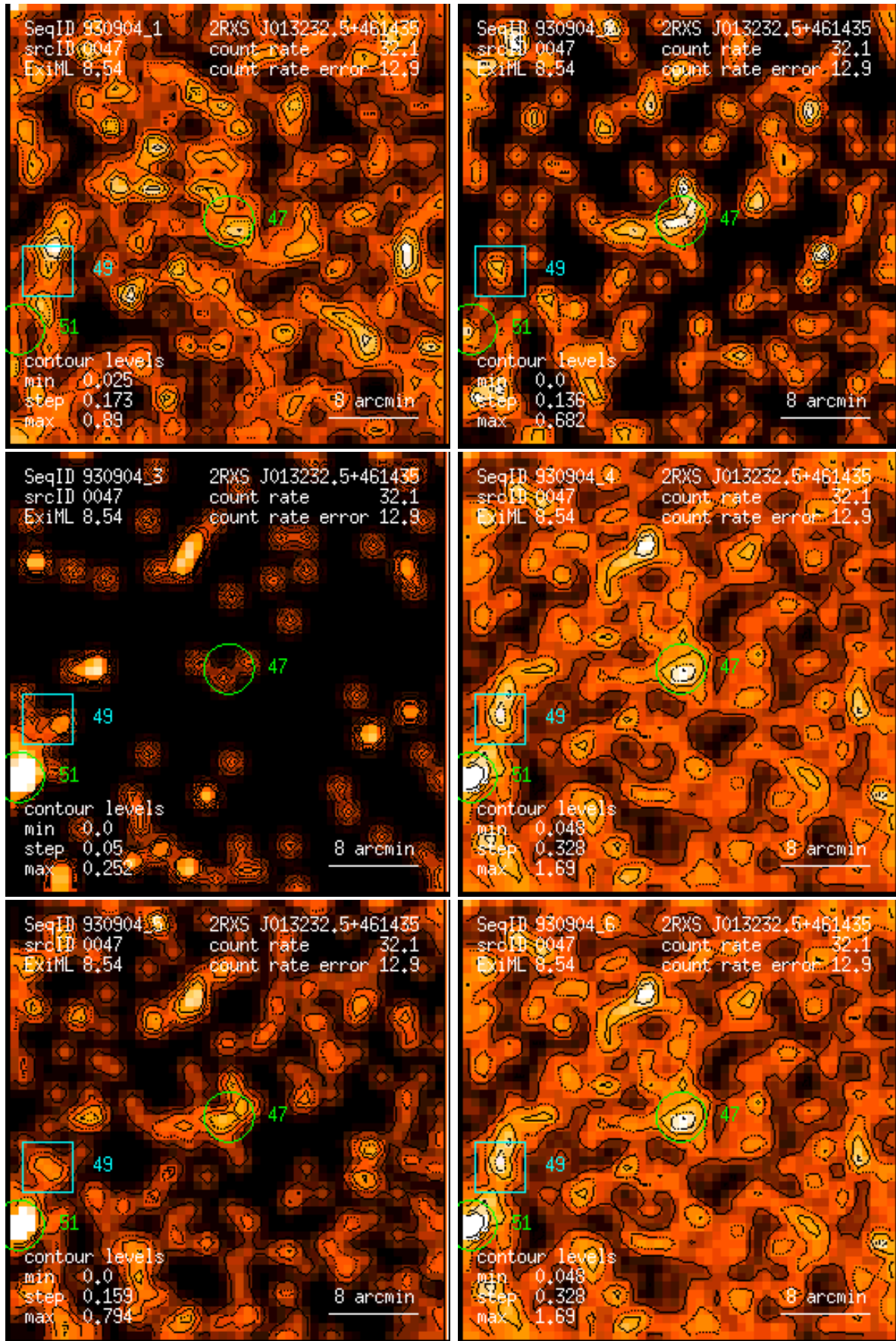
Figure 47: RASS 930904: detection 0047: band rate images, Gaussian filter: (1) PSPC channels 11 – 41, (2) 52 – 90, (3) 91 – 201, (4) 11 – 235, (5) 52 – 201, (6) 11 – 201. Broad band rates in counts/ks. Band rate contour levels in counts/ks/arcmin 2 .
