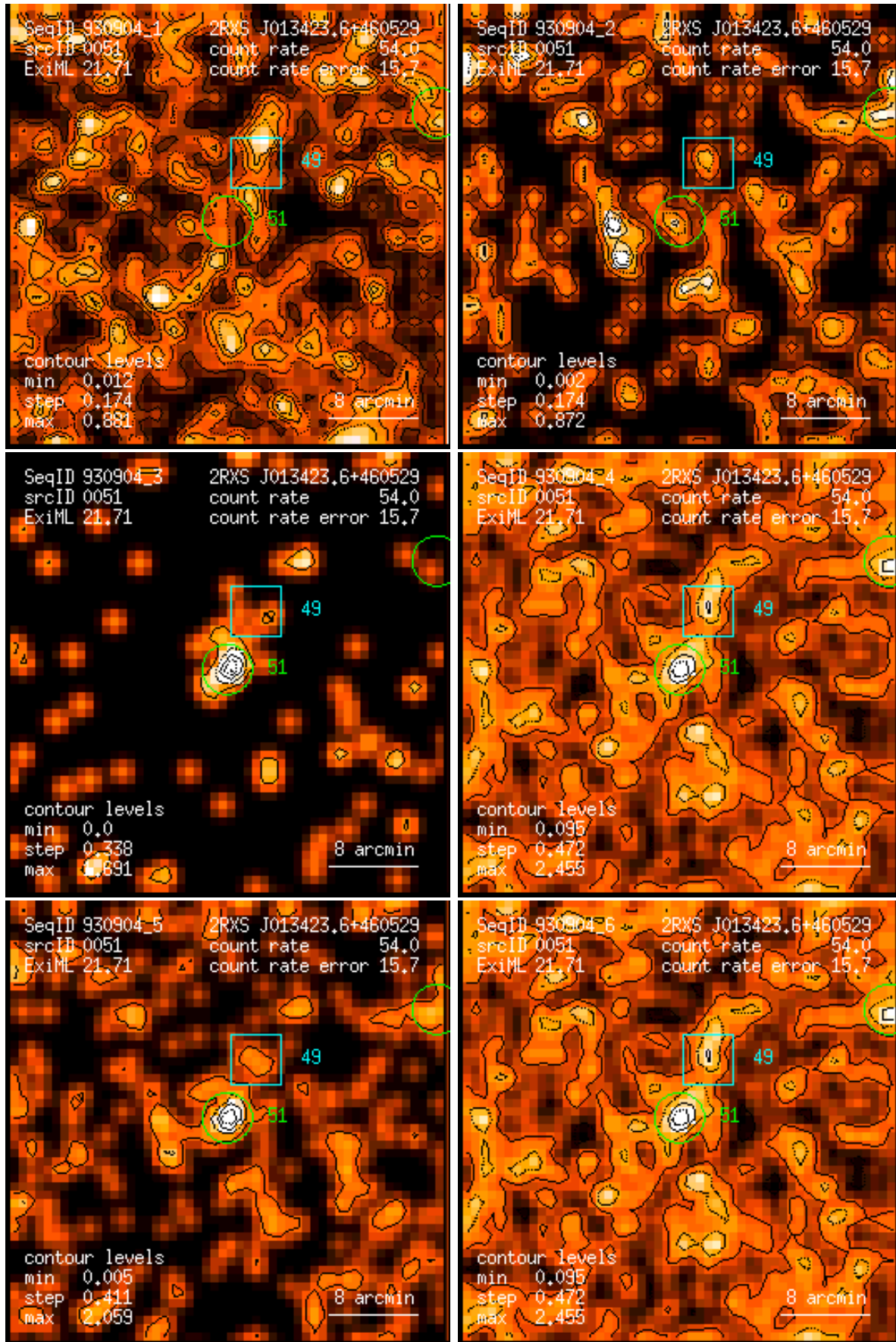
Figure 51: RASS 930904: detection 0051: band rate images, Gaussian filter: (1) PSPC channels 11 – 41, (2) 52 – 90, (3) 91 – 201, (4) 11 – 235, (5) 52 – 201, (6) 11 – 201. Broad band rates in counts/ks. Band rate contour levels in counts/ks/arcmin 2 .
