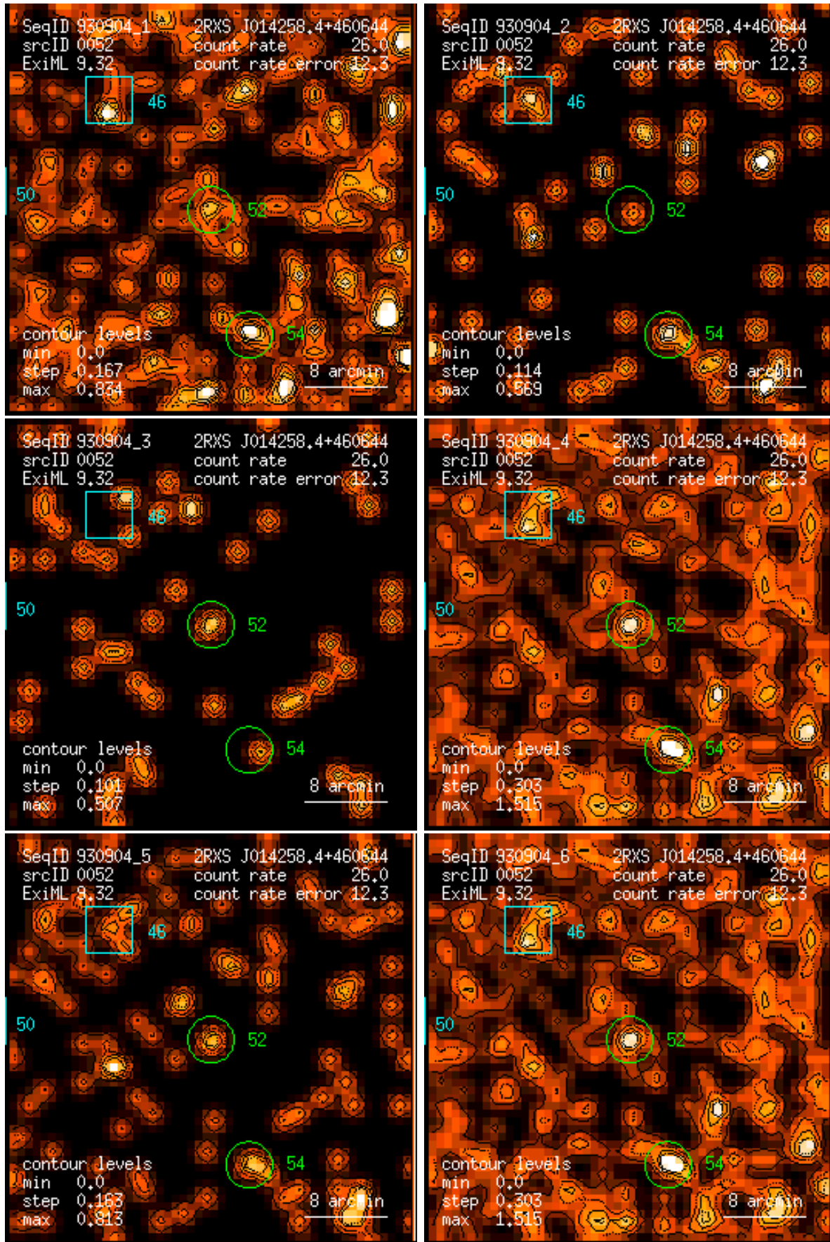
Figure 52: RASS 930904: detection 0052: band rate images, Gaussian filter: (1) PSPC channels 11 – 41, (2) 52 – 90, (3) 91 – 201, (4) 11 – 235, (5) 52 – 201, (6) 11 – 201. Broad band rates in counts/ks. Band rate contour levels in counts/ks/arcmin 2 .
