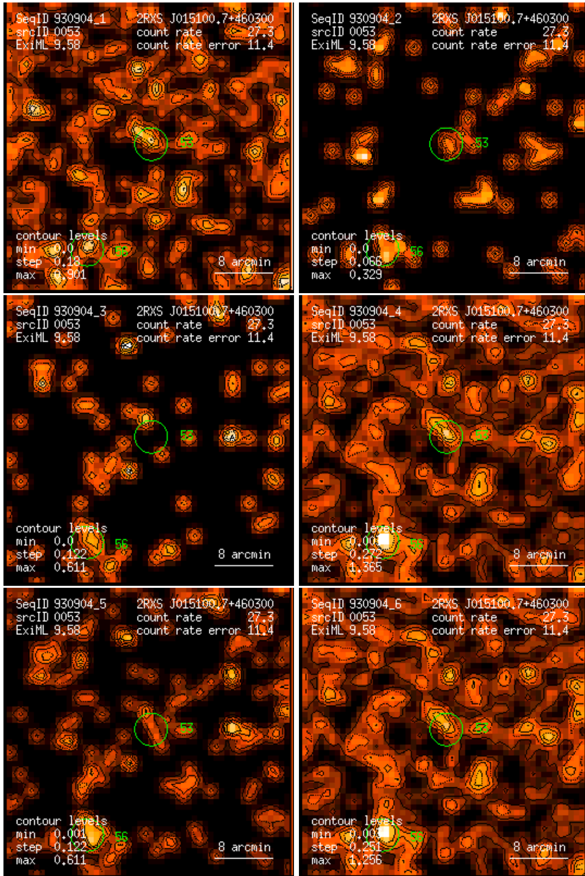
Figure 53: RASS 930904: detection 0053: band rate images, Gaussian filter: (1) PSPC channels 11 – 41, (2) 52 – 90, (3) 91 – 201, (4) 11 – 235, (5) 52 – 201, (6) 11 – 201. Broad band rates in counts/ks. Band rate contour levels in counts/ks/arcmin 2 .
