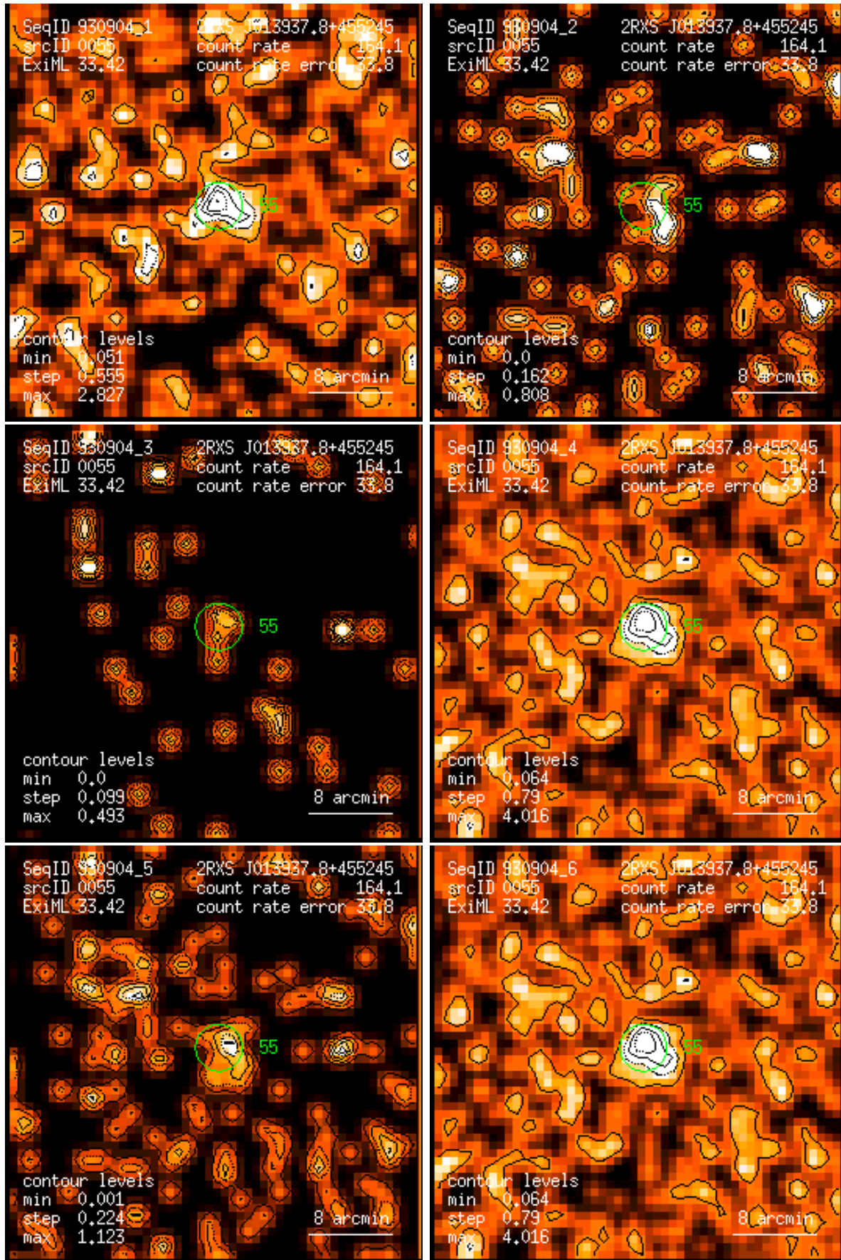
Figure 55: RASS 930904: detection 0055: band rate images, Gaussian filter: (1) PSPC channels 11 – 41, (2) 52 – 90, (3) 91 – 201, (4) 11 – 235, (5) 52 – 201, (6) 11 – 201. Broad band rates in counts/ks. Band rate contour levels in counts/ks/arcmin 2 .
