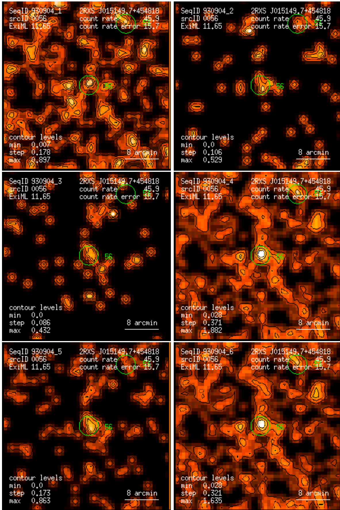
Figure 56: RASS 930904: detection 0056: band rate images, Gaussian filter: (1) PSPC channels 11 – 41, (2) 52 – 90, (3) 91 – 201, (4) 11 – 235, (5) 52 – 201, (6) 11 – 201. Broad band rates in counts/ks. Band rate contour levels in counts/ks/arcmin 2 .
