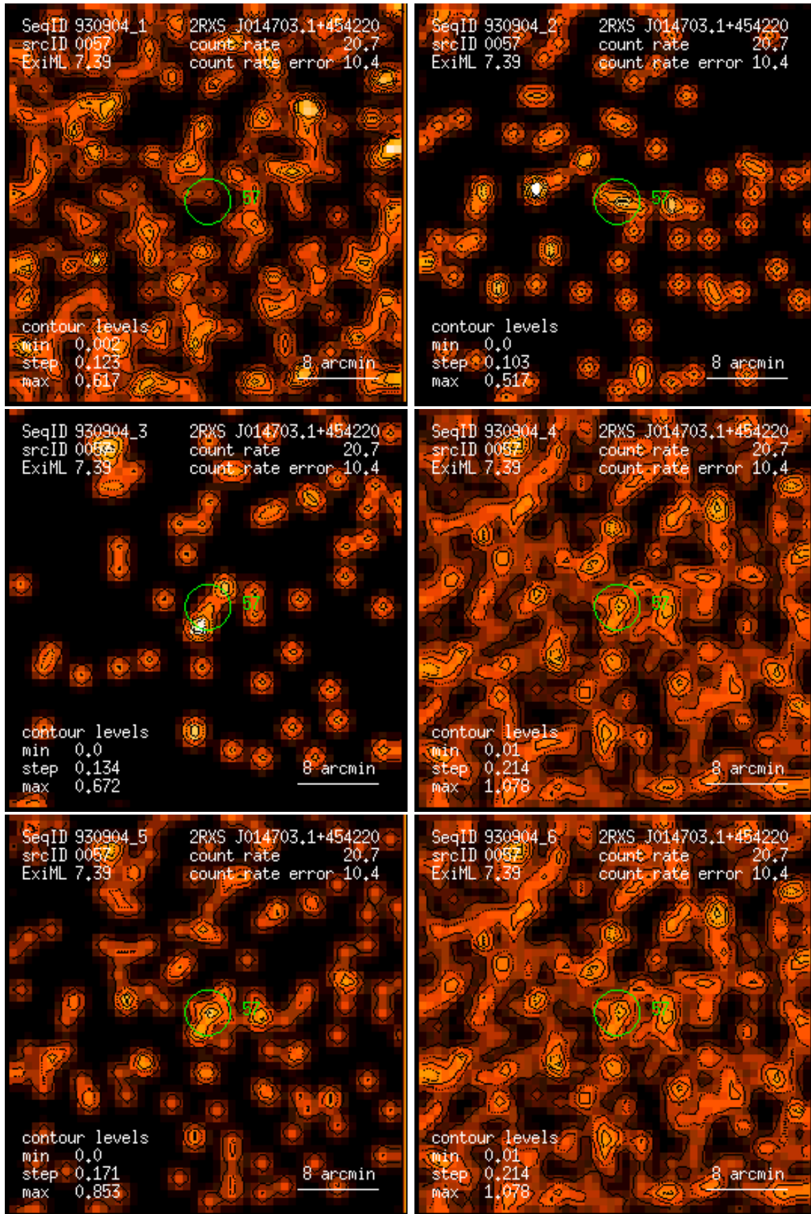
Figure 57: RASS 930904: detection 0057: band rate images, Gaussian filter: (1) PSPC channels 11 – 41, (2) 52 – 90, (3) 91 – 201, (4) 11 – 235, (5) 52 – 201, (6) 11 – 201. Broad band rates in counts/ks. Band rate contour levels in counts/ks/arcmin 2 .
