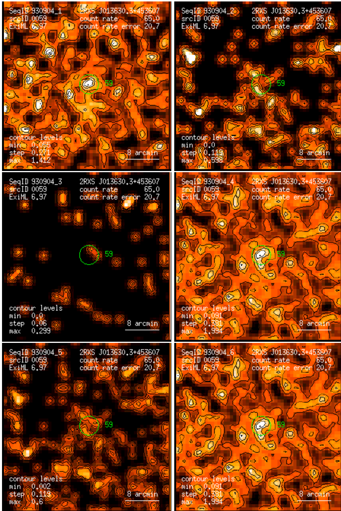
Figure 59: RASS 930904: detection 0059: band rate images, Gaussian filter: (1) PSPC channels 11 – 41, (2) 52 – 90, (3) 91 – 201, (4) 11 – 235, (5) 52 – 201, (6) 11 – 201. Broad band rates in counts/ks. Band rate contour levels in counts/ks/arcmin 2 .
