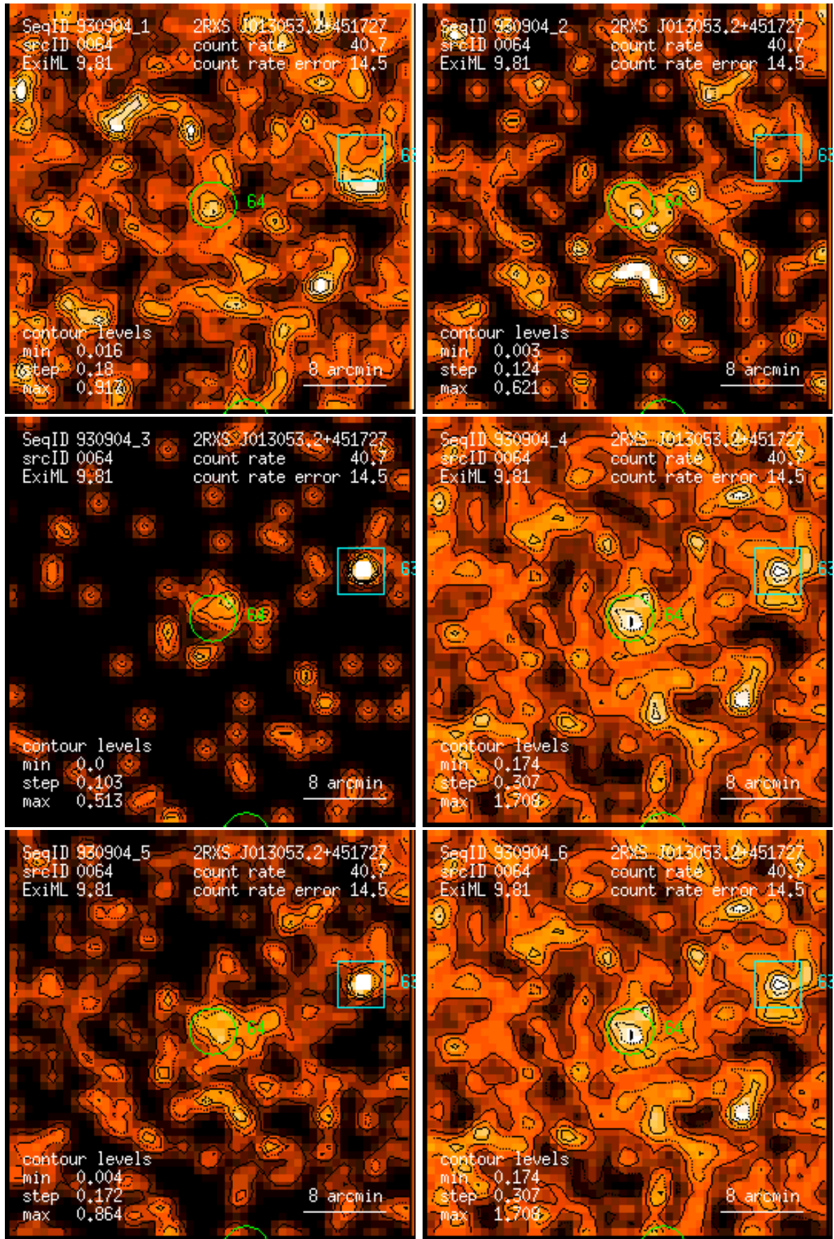
Figure 64: RASS 930904: detection 0064: band rate images, Gaussian filter: (1) PSPC channels 11 – 41, (2) 52 – 90, (3) 91 – 201, (4) 11 – 235, (5) 52 – 201, (6) 11 – 201. Broad band rates in counts/ks. Band rate contour levels in counts/ks/arcmin 2 .
